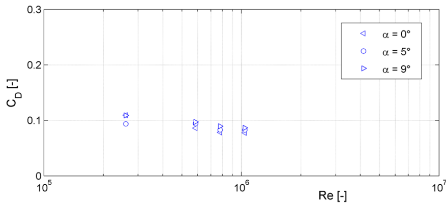
Figure 14. Drag coefficient vs. Reynolds number of the falcon model for different angles of attack \alpha . Measurements were done for different Reynolds numbers [ Re = 260\,000 ( v = 10\text{ m s}^{-1} ), Re = 585\,000 ( v = 22.5\text{ m s}^{-1} ), Re = 780\,000 ( v = 30\text{ m s}^{-1} ) and Re = 1\,040\,000 ( v = 40\text{ m s}^{-1} )]. doi:10.1371/journal.pone.0086506.g014
