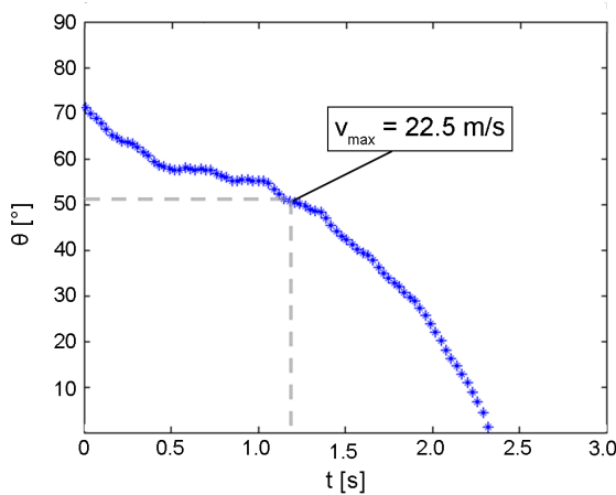
Figure 11. Variation of flight path angle \theta in the major tracking phase. The bird starts from almost vertical flight ( \theta = 90^\circ relative to the horizontal) and still had a flight path angle of \theta = 70^\circ when it entered the tracking area ( t = 0 ). The light path angle decreased then continuously until the bird pulled out ( \theta = 0^\circ ) at 2.3 s. The flight path angle is about 50.75^\circ when the bird reached the maximum velocity. doi:10.1371/journal.pone.0086506.g011
