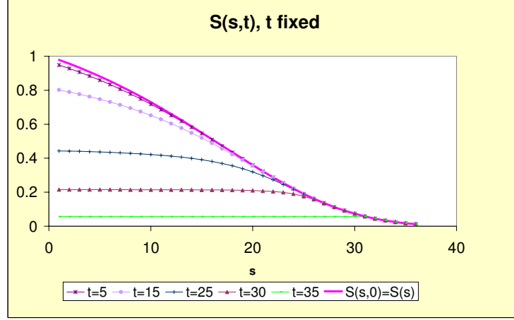
Figure 5. Sections of the joint analytical survival function, for female fixed duration.
