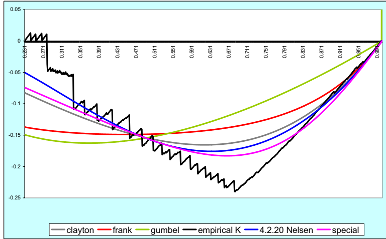
Figure 3. Graphical comparison among theoretical and empirical \lambda(z) = z - K(z) functions.
