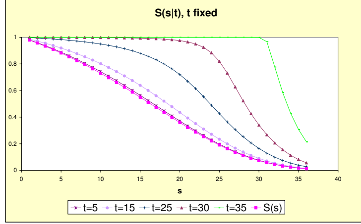
Figure 10. Male conditional survival probability for fixed female duration t .
