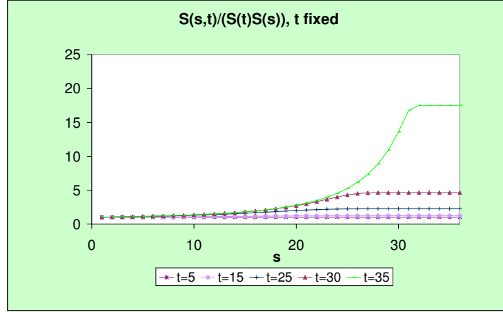
Figure 8. Sections of the association measure \psi_1(s, t) = \frac{S(s, t)}{S(s)S(t)} , for fixed female duration t .
