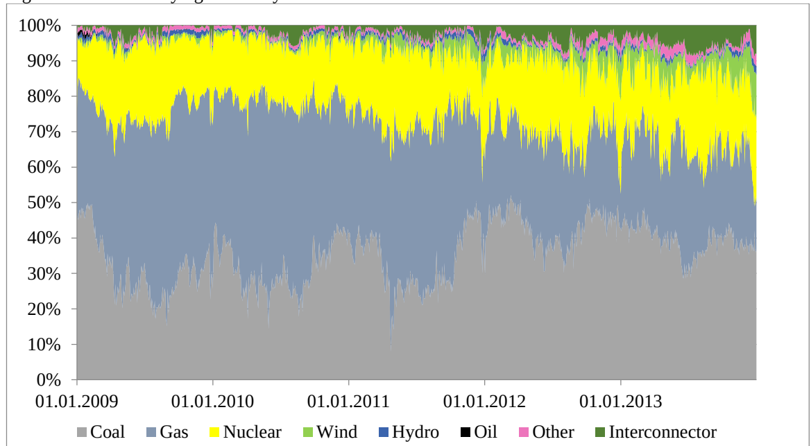
Figure 3.32: Time-varying electricity mix GB
