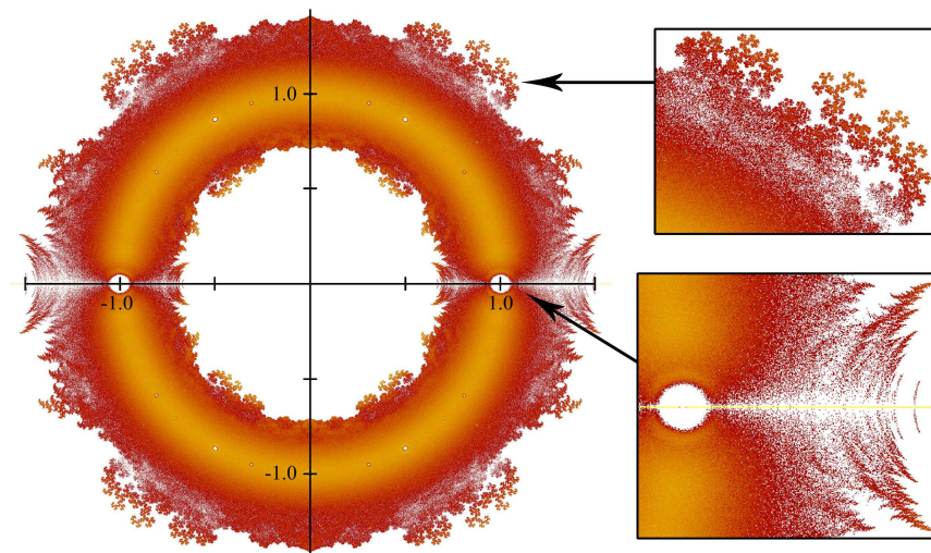
Fig. 1. Plot of complex roots for an order 24 Littlewood polynomial with \pm 1 coefficients. Areas which show self-similarity have been enlarged.
