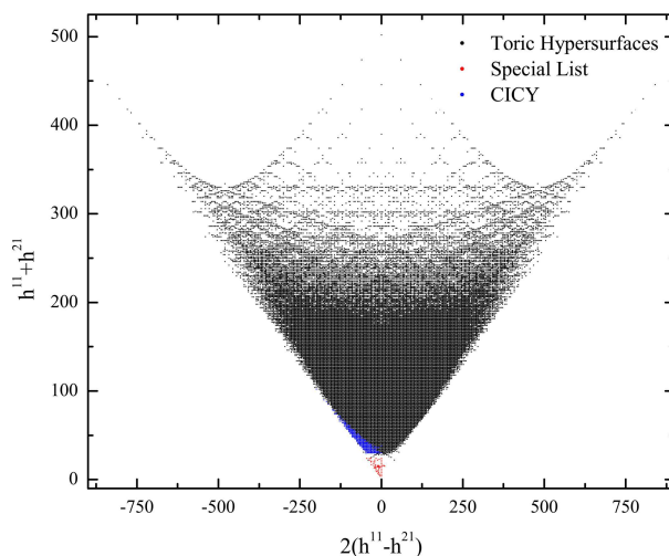
Fig. 2. A plot of the Hodge numbers for known Calabi-Yau three-folds coloured according to the list they are drawn from. The horizontal axis is 2(h^{1,1} - h^{2,1}) = \chi , the Euler characteristic; the vertical axis is \frac{1}{2}(P_{\mathcal{M}}(1) - 4) = h^{1,1} + h^{2,1} . Calabi-Yau three-folds which lie on the vertical line through the origin have \chi = 0 .
