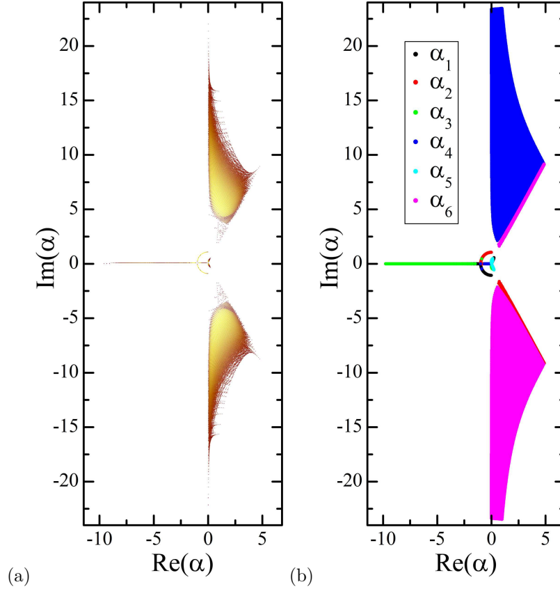
Fig. 6. (a) A plot of the density of roots for Calabi-Yau three-folds in the complex plane. Red indicates low density while yellow signifies high density. (b) A plot of the analytic roots for a sextic palindromic polynomial with vanishing linear and quintic terms of the form P = 1 + at^2 + (2 + 2b)t^3 + at^4 + t^6 where a, b take random values in the range [1, 491] .
