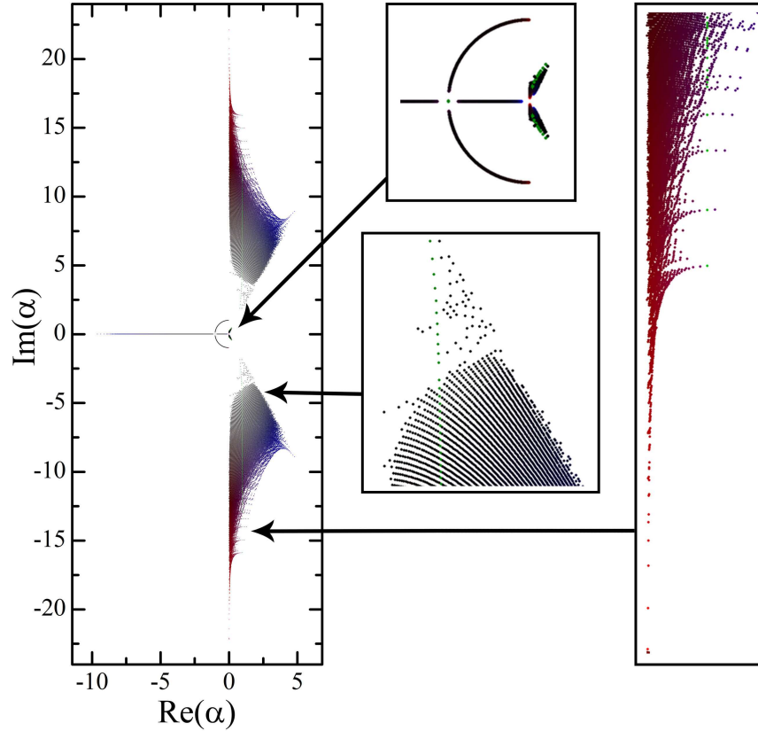
Fig. 5. A plot of the roots for known Calabi-Yau three-folds in the complex plane. Red corresponds to large values of h^{1,1} , blue to large h^{2,1} and green for h^{1,1} = h^{2,1} . Areas of interest are shown enlarged.
