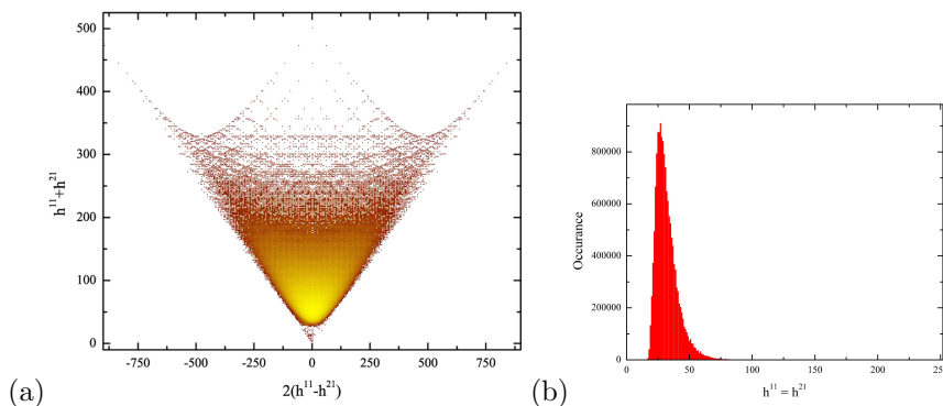
Fig. 3. (a) A plot of the density of Hodge numbers of all known Calabi-Yau three-folds. As standard, \frac{1}{2}(P_{\mathcal{M}}(1) - 4) = h^{1,1} + h^{2,1} is the ordinate while P_{\mathcal{M}}(-1) = \chi = 2(h^{1,1} - h^{2,1}) is the abscissa. In colour rendering, red indicates low density while yellow is high density. (b) A histogram plot of the self-mirror three-folds. There is a dramatic peak around (h^{1,1}, h^{2,1}) = (27, 27) in both (a) and (b).
