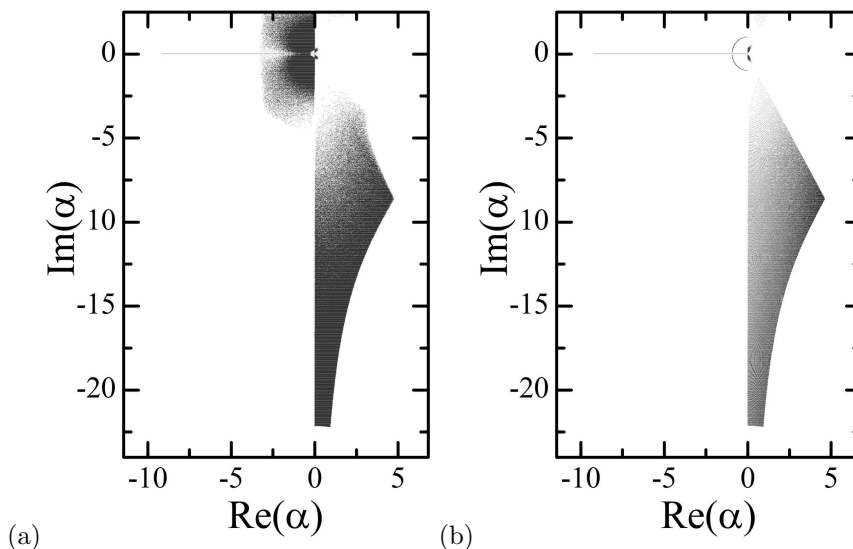
Fig. 4. (a) A plot of the roots for a sextic polynomial with vanishing linear and quintic terms of the form P = 1 + at^2 + (2 + 2b)t^3 + ct^4 + t^6 . a, b, c take random values from [1, 491] . (b) A subset of part (a) but using only palindromic polynomials.
