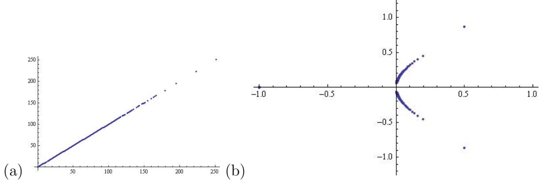
Figure 5: (a) The Hodge number of self-mirror Calabi-Yau threefolds; these have -1 as a root of the Poincaré polynomial. (b) All of the roots of the Poincaré polynomial of these self-mirrors.
