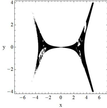
Higgsing 1
