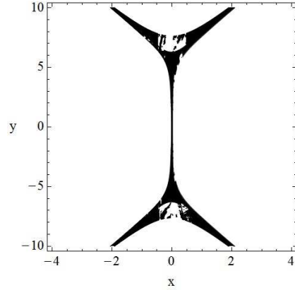
Higgsing 2
