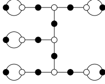
19, 1, 1, 1, 1, 1 ( \mathbb{Q} )
