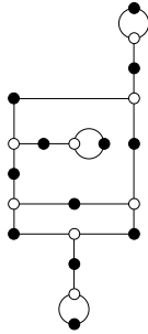
11, 7, 3, 1, 1, 1 (cubic)
