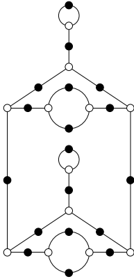
\Gamma_1(10) 10, 10, 5, 5, 2, 2, 1, 1
