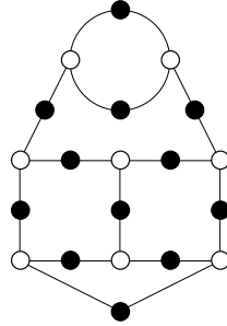
6, 5, 4, 4, 3, 2 ( \mathbb{Q} )
