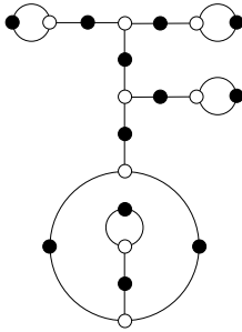
15, 5, 1, 1, 1, 1 ( \sqrt{-15} )
