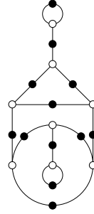
8, 6, 5, 3, 1, 1 ( \sqrt{5} )
