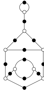
8, 6, 4, 3, 2, 1 ( \sqrt{2} )
