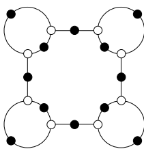
8, 8, 2, 2, 2, 2 ( \mathbb{Q} )
