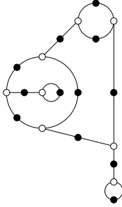
9, 6, 5, 2, 1, 1 (cubic)
