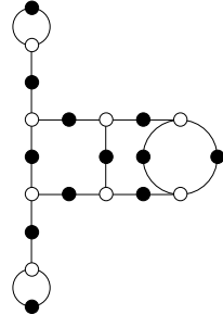
12, 4, 4, 2, 1, 1 ( \mathbb{Q} )
