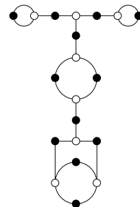
15, 3, 2, 2, 1, 1 ( \mathbb{Q} )
