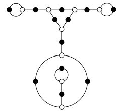
13, 5, 3, 1, 1, 1 ( \mathbb{Q} )
