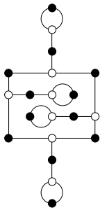
10, 10, 1, 1, 1, 1 ( \mathbb{Q} )
