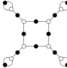
16, 4, 1, 1, 1, 1 ( \mathbb{Q} )
