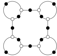
\Gamma_0(8) \cap \Gamma(2) 8, 8, 2, 2, 2, 2
