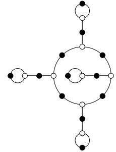
13, 7, 1, 1, 1, 1 ( \mathbb{Q} )
