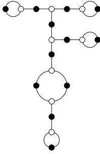
18, 2, 1, 1, 1, 1 ( \sqrt{-3} )
