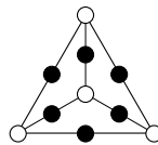
\Gamma_0(3) 3, 3, 3, 3
