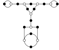
14, 3, 3, 2, 1, 1 ( \mathbb{Q} )
