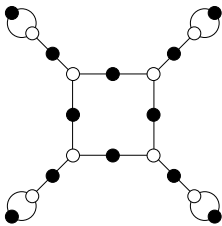
\Gamma_0(16) 16, 4, 1, 1, 1, 1
