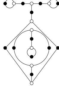
10, 6, 5, 1, 1, 1 (cubic)
