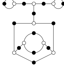
11, 5, 4, 2, 1, 1 (cubic)
