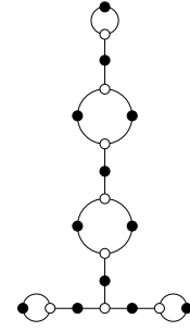
17, 2, 2, 1, 1, 1 ( \sqrt{17} )
