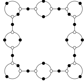
\Gamma(16; 8, 2, 2) 16, 16, 2, 2, 2, 2, 2, 2, 2, 2
