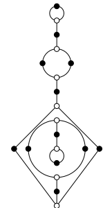
9, 6, 5, 2, 1, 1 (cubic)
