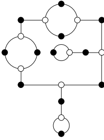
9, 9, 2, 2, 1, 1 (cubic)
