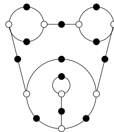
7, 6, 6, 2, 2, 1 ( \mathbb{Q} )
