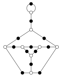
7, 5, 4, 4, 3, 1 ( \mathbb{Q} )
