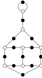
8, 4, 4, 4, 3, 1 ( \mathbb{Q} )
