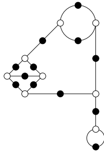
9, 6, 3, 3, 2, 1 (cubic)
