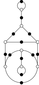
9, 6, 4, 3, 1, 1 ( \mathbb{Q} )
