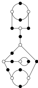
9, 7, 3, 2, 2, 1 (cubic)
