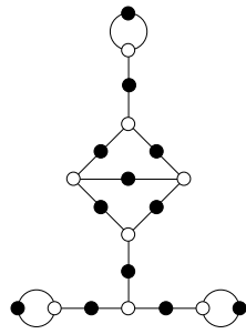
15, 3, 3, 1, 1, 1 ( \mathbb{Q} )
