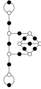
11, 5, 3, 3, 1, 1 ( \sqrt{5} )
