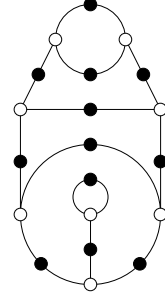
6, 6, 5, 4, 2, 1 ( \mathbb{Q} )
