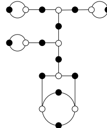
16, 3, 2, 1, 1, 1 ( \sqrt{-2} )
