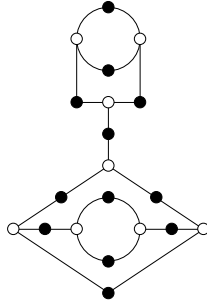
8, 5, 4, 3, 2, 2 ( \mathbb{Q} )
