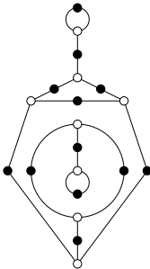
7, 7, 5, 3, 1, 1 ( \sqrt{21} )
