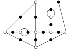
7, 7, 4, 4, 1, 1 ( \sqrt{-7} )
