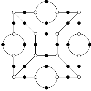
\Gamma(12; 6, 1, 2) 12, 6, 6, 6, 6, 4, 2, 2, 2, 2
