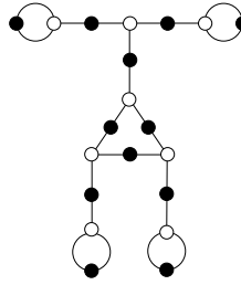
17, 3, 1, 1, 1, 1 ( \mathbb{Q} )
