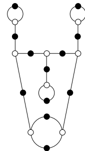
11, 8, 2, 1, 1, 1 (cubic)
