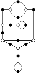
9, 8, 3, 2, 1, 1 (cubic)
