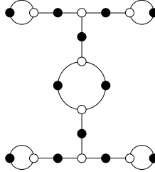
18, 2, 1, 1, 1, 1 ( \mathbb{Q} )
