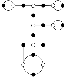
16, 3, 2, 1, 1, 1 ( \sqrt{-2} )
