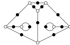
7, 7, 5, 3, 1, 1 ( \sqrt{21} )
