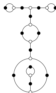
14, 5, 2, 1, 1, 1 (cubic)
