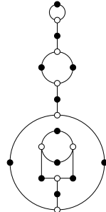
9, 7, 3, 2, 2, 1 (cubic)
