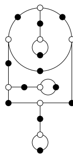
8, 7, 6, 1, 1, 1 ( \sqrt{-3} )
