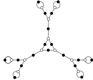
\Gamma(27; 27, 3, 3) 27, 3, 1, 1, 1, 1, 1, 1
