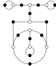
11, 6, 4, 1, 1, 1 ( \sqrt{33} )
