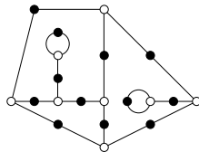
7, 7, 4, 4, 1, 1 ( \sqrt{-7} )
