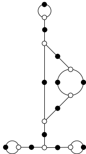
15, 4, 2, 1, 1, 1 ( \sqrt{-15} )
