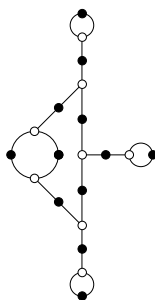
14, 5, 2, 1, 1, 1 ( \mathbb{Q} )
