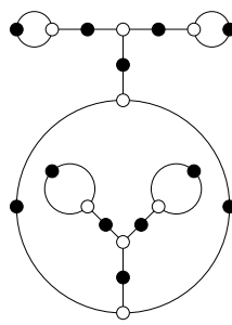
10, 10, 1, 1, 1, 1 ( \sqrt{5} )
