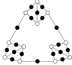
\Gamma(9; 3, 1, 3) 9, 9, 3, 3, 3, 3, 3, 3
