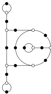
11, 6, 4, 1, 1, 1 ( \sqrt{33} )
