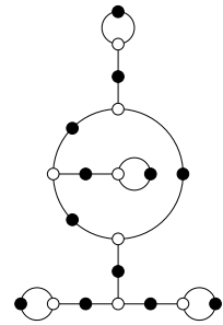
14, 6, 1, 1, 1, 1 ( \sqrt{-3} )
