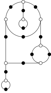
8, 6, 6, 2, 1, 1 ( \sqrt{-3} )
