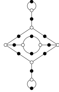
10, 5, 5, 2, 1, 1 ( \sqrt{5} )
