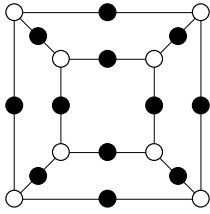
\Gamma(4) 4, 4, 4, 4, 4, 4
