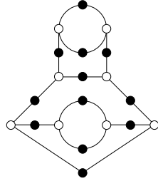
6, 6, 4, 4, 2, 2 ( \mathbb{Q} )
