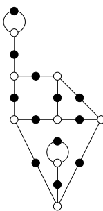
8, 7, 4, 3, 1, 1 ( \sqrt{-6} )
