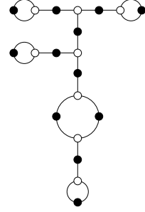
18, 2, 1, 1, 1, 1 ( \sqrt{-3} )
