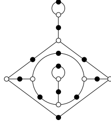
6, 6, 5, 5, 1, 1 ( \sqrt{3} )
