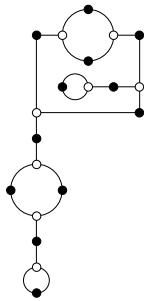
11, 7, 2, 2, 1, 1 ( \sqrt{-7} )
