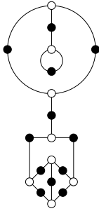
8, 5, 4, 3, 3, 1 ( \sqrt{10} )
