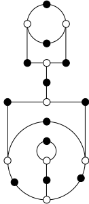
9, 6, 3, 3, 2, 1 (cubic)
