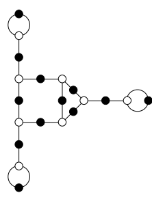
14, 4, 3, 1, 1, 1 ( \mathbb{Q} )
