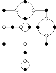
9, 9, 2, 2, 1, 1 (cubic)
