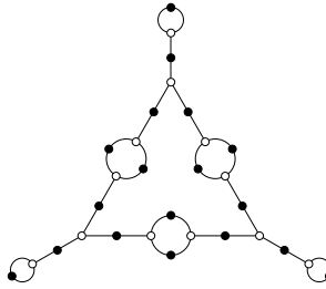
\Gamma_0(18) 18, 9, 2, 2, 2, 1, 1, 1
