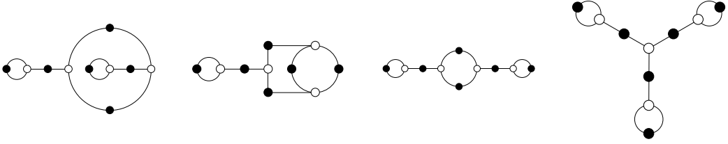
\Gamma_1(5) 5, 5, 1, 1
