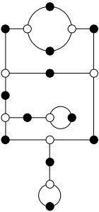
9, 7, 4, 2, 1, 1 ( \sqrt{-7} )
