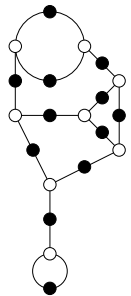
9, 5, 4, 3, 2, 1 (cubic)
