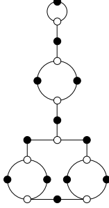
12, 5, 2, 2, 2, 1 ( \mathbb{Q} )
