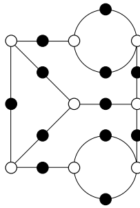
7, 5, 5, 3, 2, 2 ( \mathbb{Q} )
