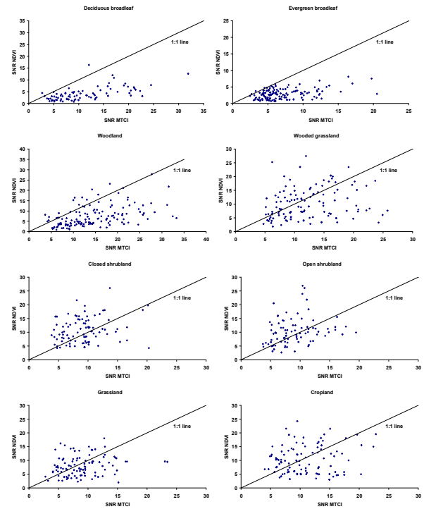
Figure 2. Relationship between MTCI SNR and NDVI SNR for eight land cover classes using iterative polynomial fitting.
