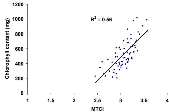
Figure 5. Relationship between MTCI and chlorophyll content for the study site at MERIS spatial resolution.
