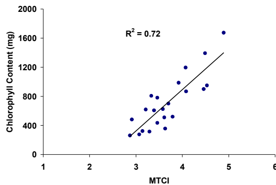
Figure 3: Relationship between MTCI derived from CASI data and chlorophyll content derived from ground data for all sampling plots in the study site.
