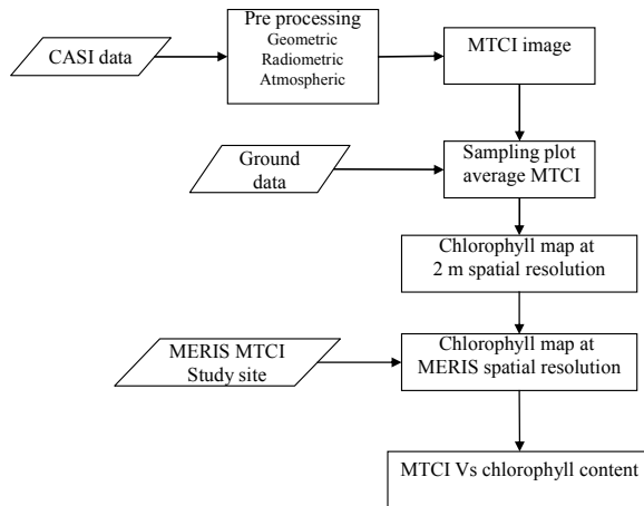
Figure 2. Methodology for MTCI validation.
