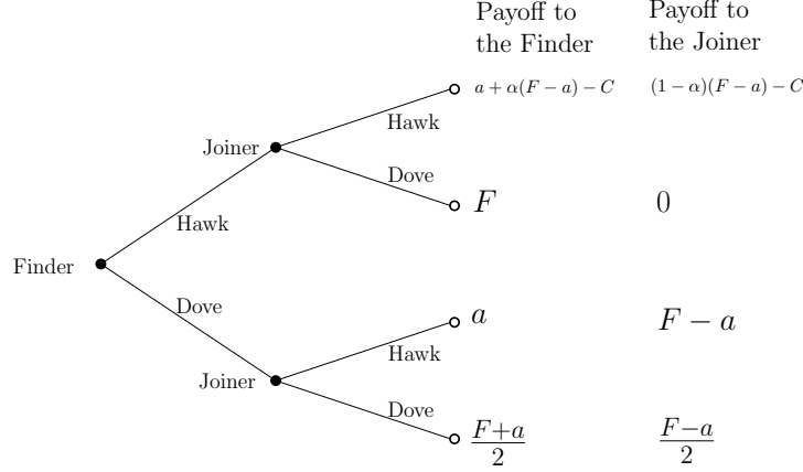
Figure 1: The sequential Finder-Joiner game in extensive form.
