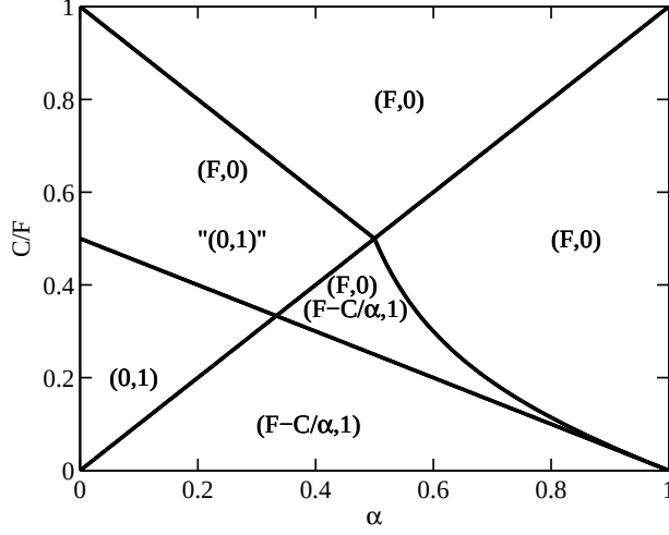
Figure 2: ESSs of the game for the asymmetric information case, where all terms are as defined in Table 1. The label “(0, 1)” denotes a region where there is an ESS of (0, 1) for the case of mistakes of the first kind (Finder plays Hawk for small values of a ). The label (0, 1) denotes a region where there is an ESS of (0, 1) for either kind of mistakes.
