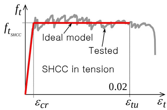
Fig.2. Tensile stress-strain curve of SHCC
