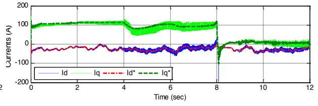
b) Wind turbine inverter d- and q-axis currents
