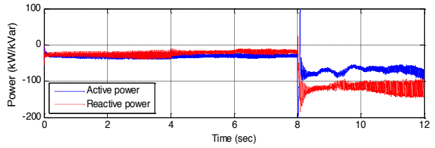
f) Active and reactive power of the microturbine
