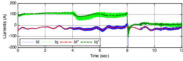
a) Solar inverter d- and q-axis currents
