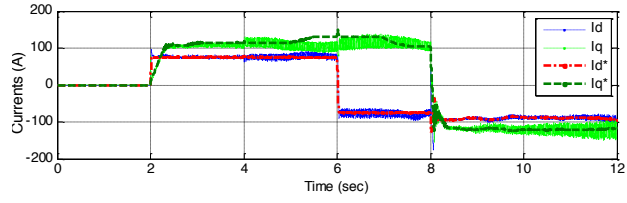
c) Battery inverter d- and q-axis currents
