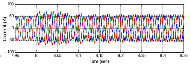
j) Three-phase load current at Bus 8
