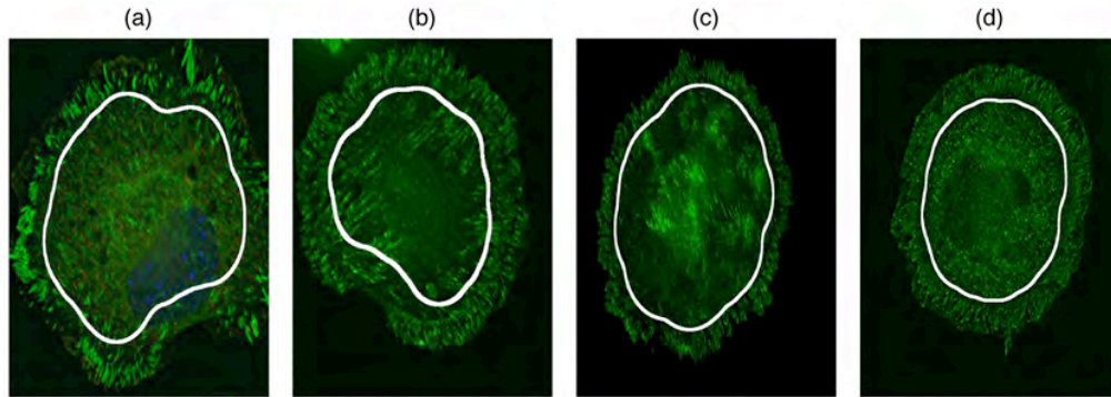
Fig. 4. The outer ring boundary overlaid on the original images. Notice how the outer ring is better located in some cells (a, c, d) than others (b). This is due to the nature of the cell in terms of shape and intensity distribution.
