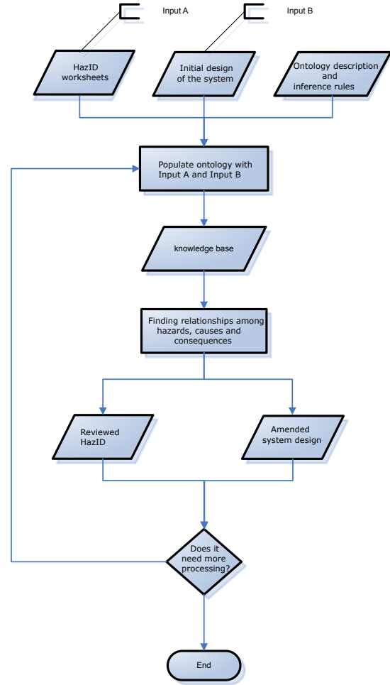
Figure 5: Control flow diagram of our method
