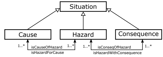
Figure 1: Examples of concepts that are part of our ontology
