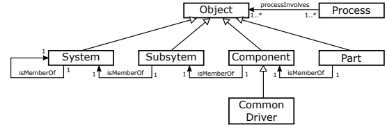
Figure 2: Part of Ontology
