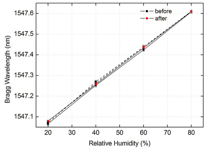
Fig. 8. Resistance of the FBG based humidity sensor to the presence of the alkaline pore water. RH measurements were performed using the climate chamber (Memmert CTC256) for increasing and decreasing humidity levels and the measurement of the Bragg wavelength of the PI-coated FBG before and after immersion in the prepared alkaline solution [16].
