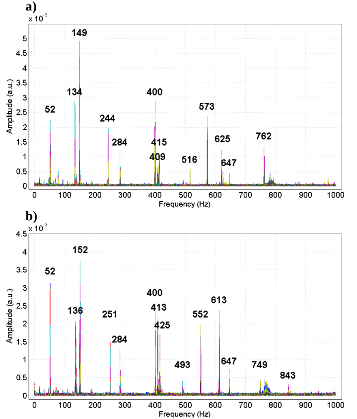
Fig. 8. FFT spectra calculated for captured signals from experimental tests in water on blade 1 (spectrum (a)) and blade 5 (spectrum (b)).
