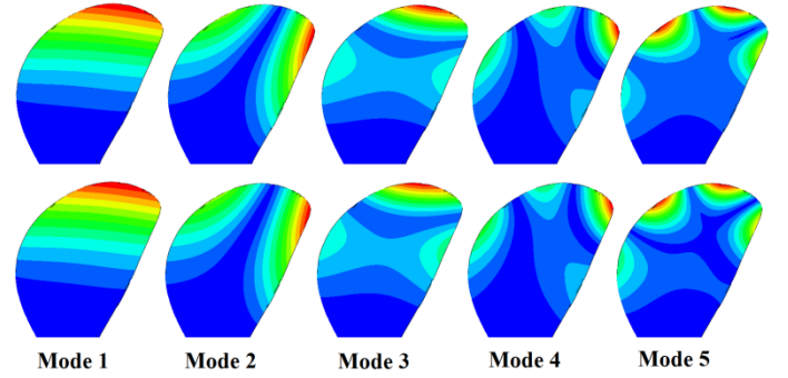
Fig. 5. Illustration of the mode shapes of the first 5 natural frequencies for blade 5 of the propeller studied in this simulation. Top row shows the mode patterns obtained in air and the bottom row are those captured in water.
