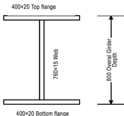
Fig. 4. Cross section of the transverse girders
