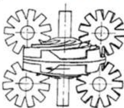
Cylindrical Screw – Planar Gaterotors
