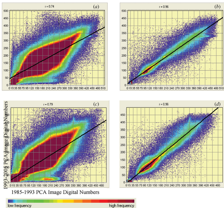
Figure 4. (a), (c) Linear regression diagram for PCA of July 1985–1993 and 1993–2005. (b), (d) The same image pairs following radiometric normalization results using PIFs.
