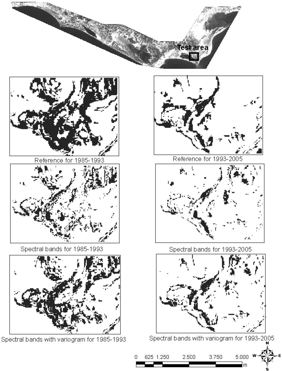
Figure 8. Comparison of CVA results for spectral bands of Landsat TM data with and without variogram outputs.
