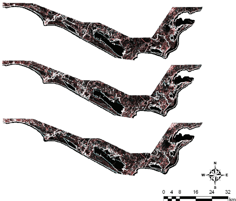
Figure 6. Variogram texture for 1985, 1993 and 2005 Landsat TM images.
