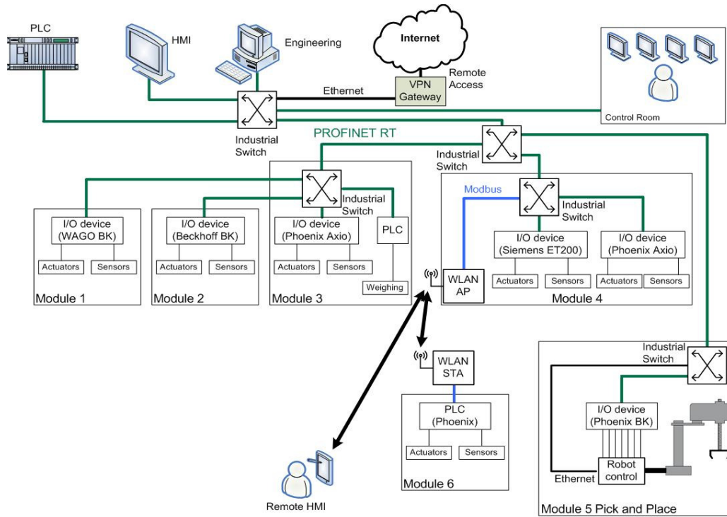
Figure 3. Network Architecture of the LMF
