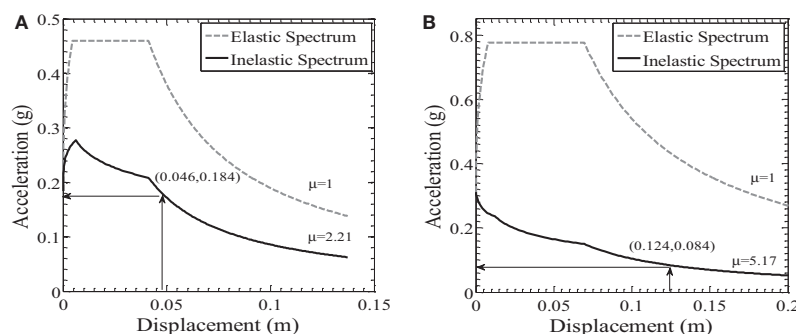
FIGURE 11 | Determination of required F_{yt}/m strengths for the (A) 10/50 seismic hazard level and (B) 2/50 seismic hazard level.
