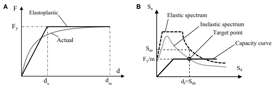
FIGURE 2 | N2 method: (A) equivalent bilinear capacity curve; (B) determination of target point (case where T \geq T_c ).
