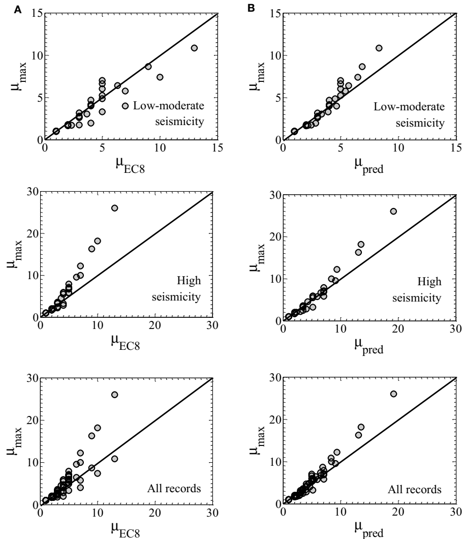
FIGURE 5 | Correlation between calculated \mu_{\max} and analytical predictions (A) by EC8 formula; (B) by proposed formulae.
