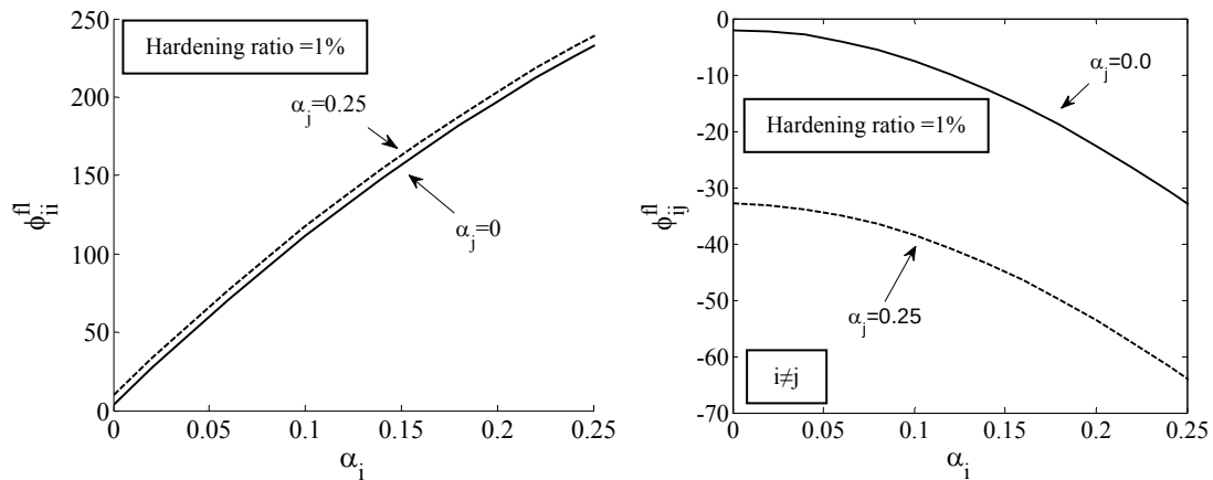
Figure 8. Variation of the normalized flexural flexibility matrix coefficients with the yielding penetration coefficients for hardening ratio 1% and uniform stiffness distribution in the inelastic zones.
