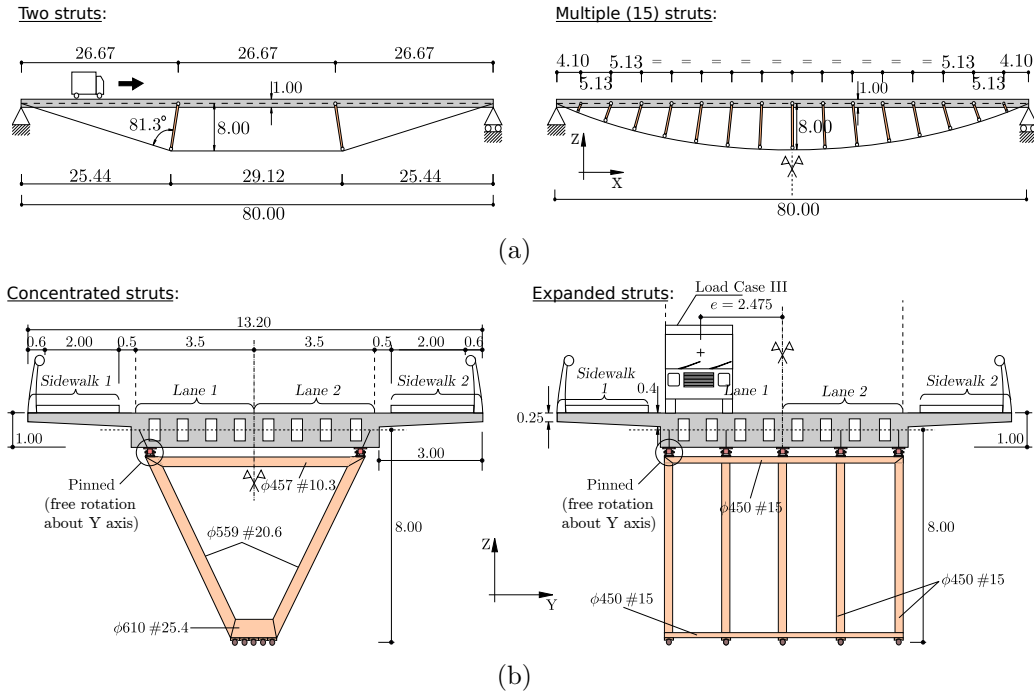
Figure 2: UD-CSBs configuration: (a) elevation with two or multiple (15) diverting struts; (b) cross section with concentrated or expanded struts, including the Load Case in which the vehicle has the maximum eccentricity in the bridge with two road lanes. Units in metres, except the steel struts (diameter \phi and thickness #) that are in millimetres.
