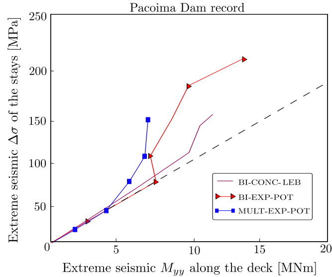
Figure 8. Maximum absolute stress variation in the cable-system span versus the extreme vertical bending moment along the deck for different amplification factors and bridge typologies. Results shown for the Pacoima Dam record using various scale factors.
