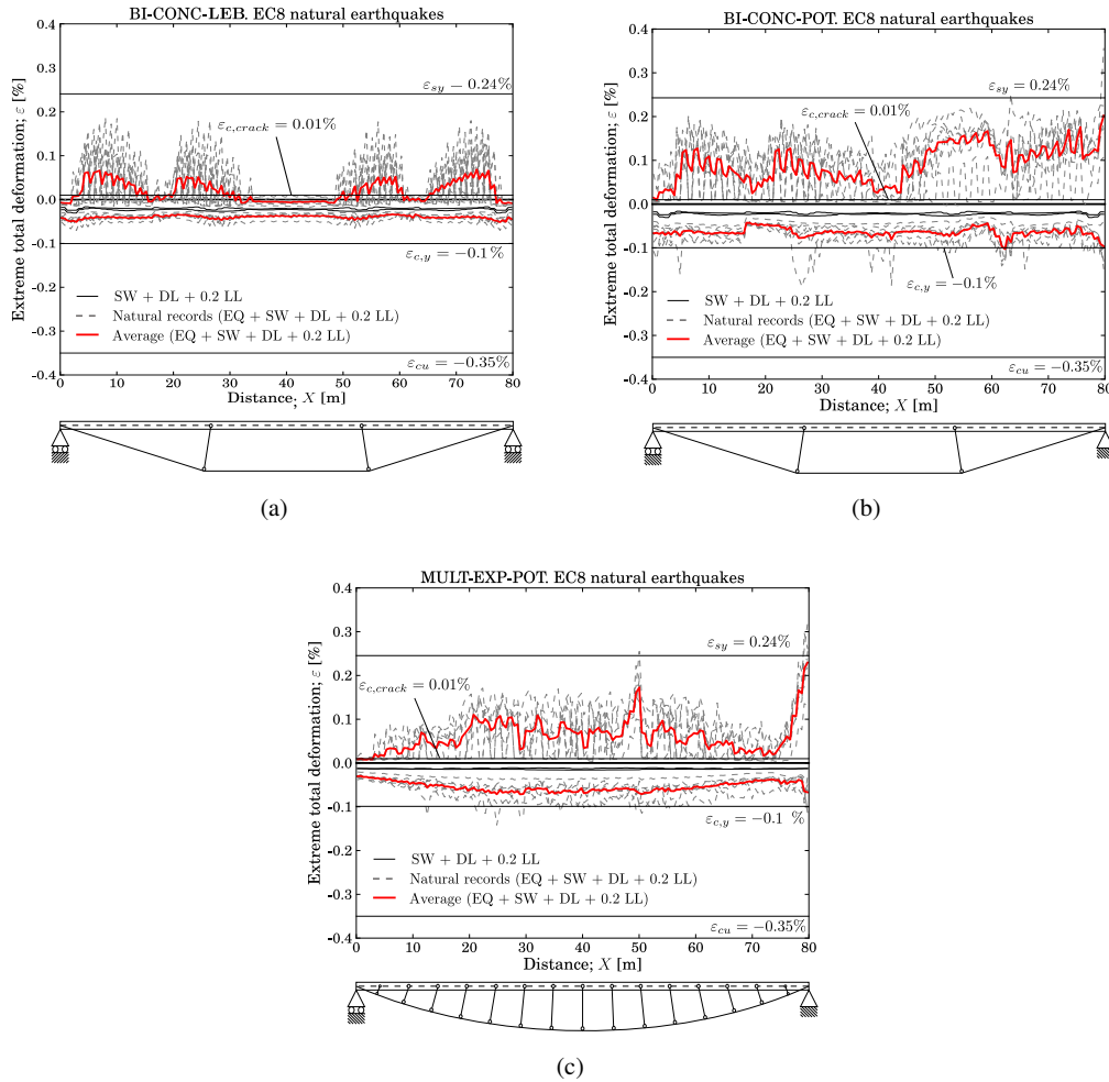
Figure 14. Distribution of the extreme total strain [%] of the deck along its length (Earthquake (EQ) + Self-Weight (SW) + superimposed Dead-Load (DL) + 20% Live-Load (LL)) with each natural record included in the set of Eurocode 8 seismic action. Concrete cracking, elastic and ultimate limits strains are included. (a) Two struts and LEB supports; (b) two struts and POT bearings (scheme a); and (c) multiple struts and POT bearings.
