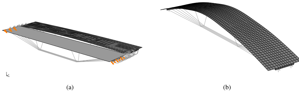
Figure 5. Fundamental vibration modes in models with different support conditions: (a) model with laminated elastomeric bearings (LEB): transverse rigid body displacement. T_1 = 1.43 s; (b) model with pot bearings (POT), classical layout: first order vertical flexure of the deck. T_1 = 1.28 s
