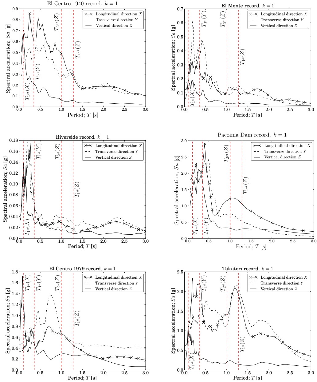
Figure 6. Longitudinal ( X ), transverse ( Y ) and vertical ( Z ) spectra of the unscaled ( k = 1 ) benchmark records. The most important vibration periods of the model with two expanded struts and POT supports (Scheme a) are also represented with different vertical dashed lines. The other typologies are not included as the first modes are similar.
