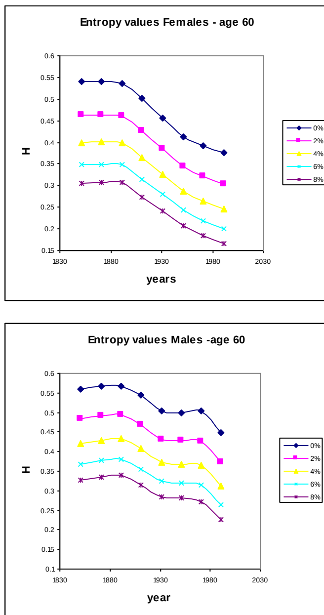
Figure 2: Entropy values for different English life tables at different rates of interest for both females and males at age 60
