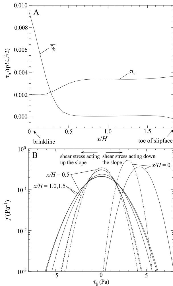
Figure 14. Bed shear stress acting on the slip face as predicted by the 3-D large eddy simulation (LES) model of Omidyeganeh et al. [2013]. (a) Plot of the mean, \bar{\tau}_b , and standard deviation, \sigma_\tau , of turbulent bed shear stresses, normalized by the density of air, \rho , and the square of the far-field velocity, U_\infty , as a function of horizontal distance from the brinkline along the dune centerline, x . (b) Frequency of bed shear stress predicted by the model for four slip-face locations ( x/H = 0, 0.5, 1.0, 1.5 ) and two values of the far-field velocity ( U_\infty = 25 \text{ m s}^{-1} (dashed curve) and 30 \text{ m s}^{-1} (solid curve)). Positive values act down the slope, i.e., with gravity, while negative values act up the slope.
