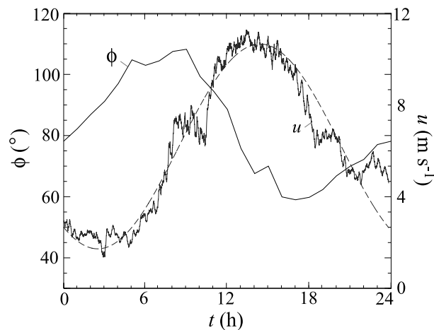
Figure 3. Average hourly wind direction ( \phi ) at Parnaíba airport (located 130 km west of Jericoacoara) during November (period of record: 1943–2013), and 5 min average wind speed ( u ) measured 0.75 m above the ground at the crest of the small dune on 8 November 2013. The dashed line is a sinusoidal fit to the wind speed (see section 3 for further discussion).
