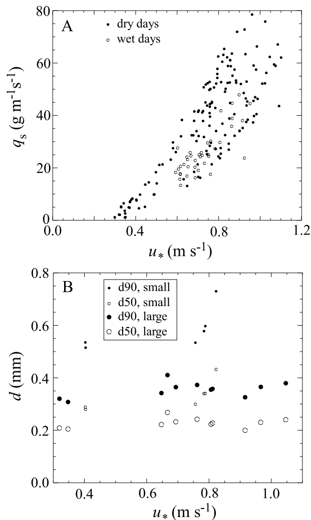
Figure 4. Measurements of flux and texture of sand in transport over the brinkline. (a) Mean unit sediment flux, q_s , over the brinkline as a function of shear velocity, u_* . Open circles indicate data from 4 and 5 November, the 2 days when significant soil moisture was present. (b) Plot of the median grain diameter, d_{50} , and the grain diameter of the 90th percentile, d_{90} , of sand in transport over the brinkline, as a function of shear velocity for the large and small dune experiment locations.
