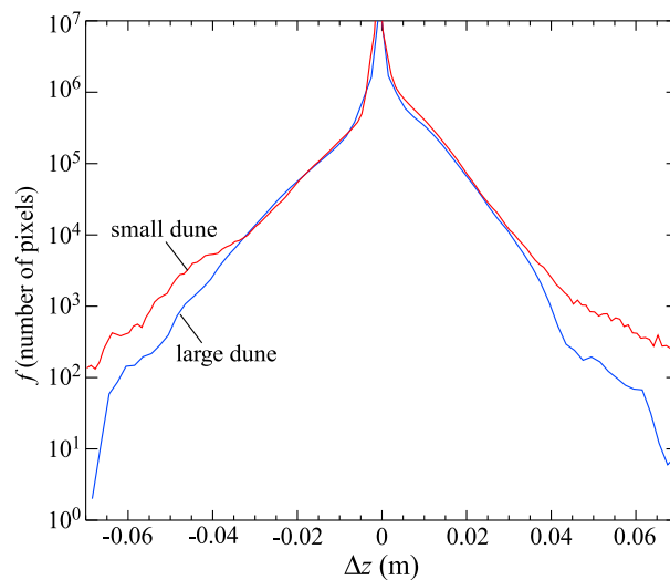
Figure 7. Plots of the frequency of occurrence of elevation changes, \Delta z , from the large (blue curve) and small (red curve) dunes. These data show that the vast majority of grain flows involve local elevation changes in the 20–60 mm range. Grain flows are slightly thicker, on average, on the smaller dune. Note that magnitudes of change below approximately 5 mm are not significant (i.e., they are indistinguishable from zero).
