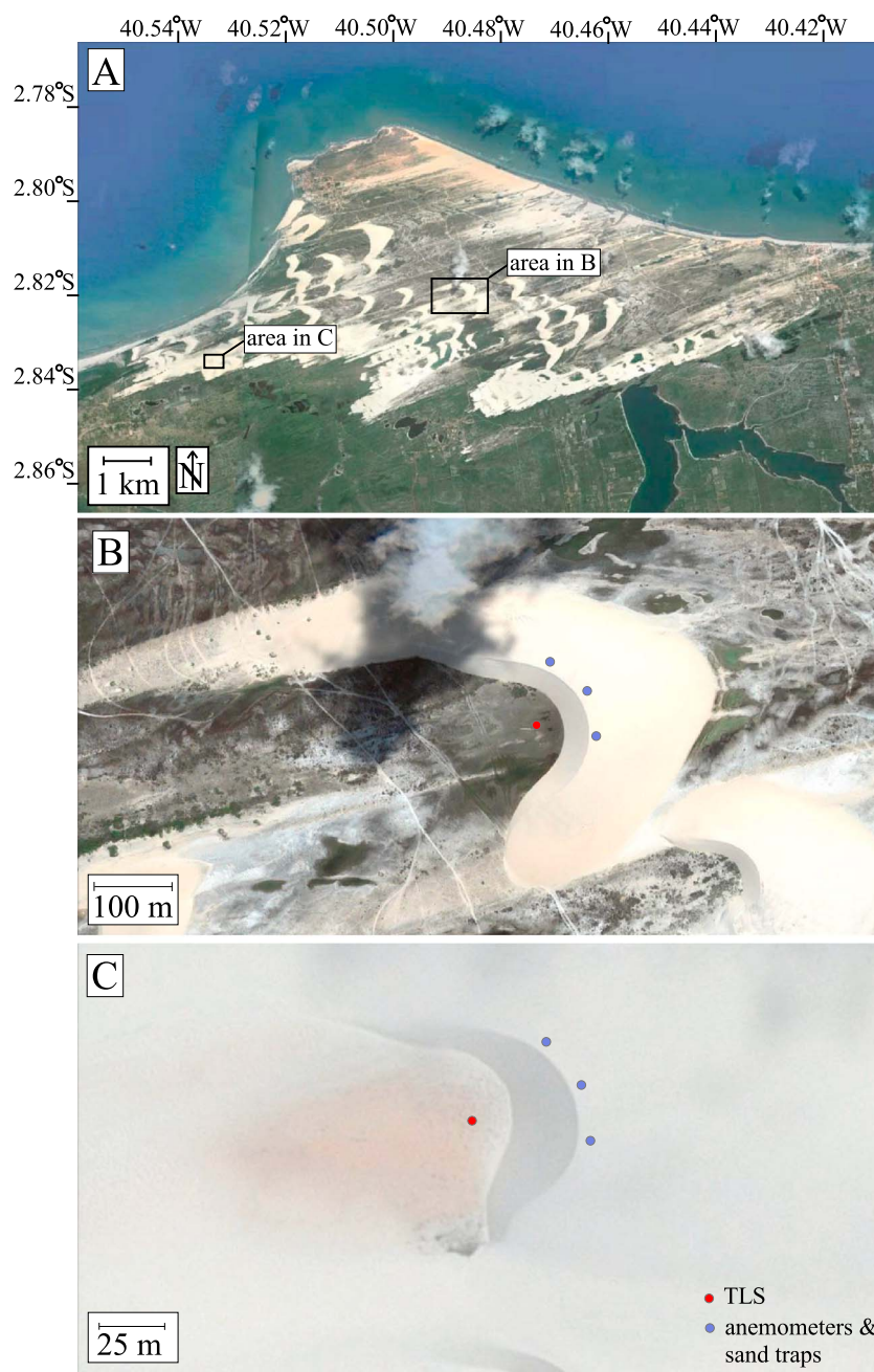
Figure 2. Aerial photographs of the study site: (a) the Jericoacoara dune field, (b) the larger of the two dunes in the study, and (c) the smaller of the two dunes. The locations of the TLS (red dots) and anemometers and sand traps (blue dots) are also shown. Image source:
