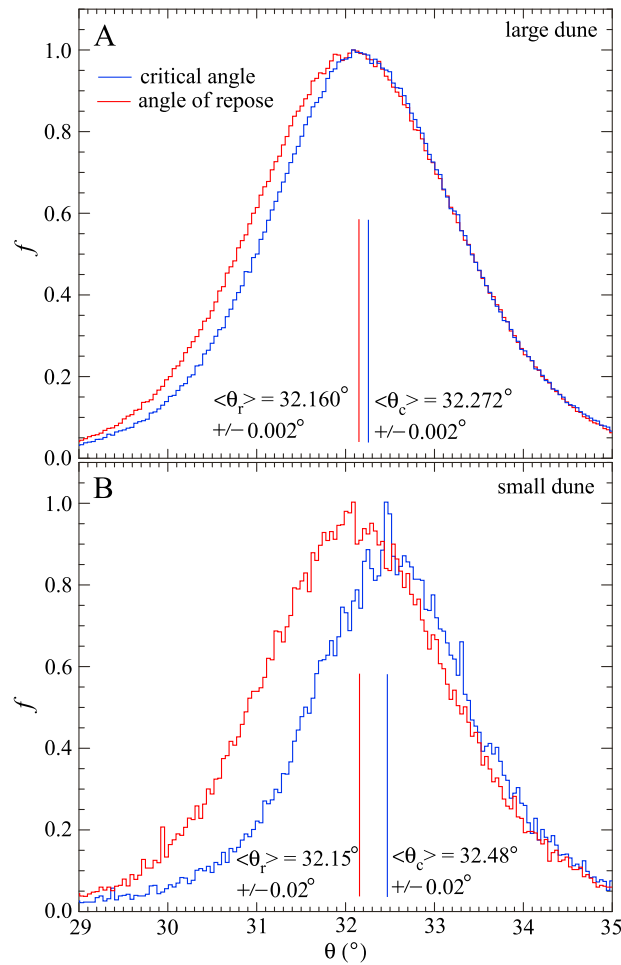
Figure 11. Example distributions (i.e., plots of relative frequency) of the critical angle (in blue) and the angle of repose (in red) measured for the (a) large and (b) small dunes. Also shown are the mean values (with uncertainties) for each distribution.
