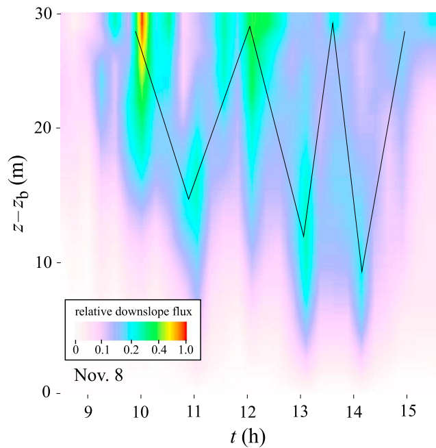
Figure 13. Color map constructed from all of the flux maps obtained on 8 November (example in Figure 6d), illustrating the average unit sediment flux by grain flows as a function of the height above the base of the slip face, z - z_b (where z_b is the elevation of the base) and time during the day. This map illustrates the cyclic nature of the storage-and-release process, with periods of steepening/storage on the top portion of the slope followed by advective transport of a portion of those deposits down the slope. The black lines are included simply to highlight the oscillating nature of the flux as the slope shifts from storage to release phases.
