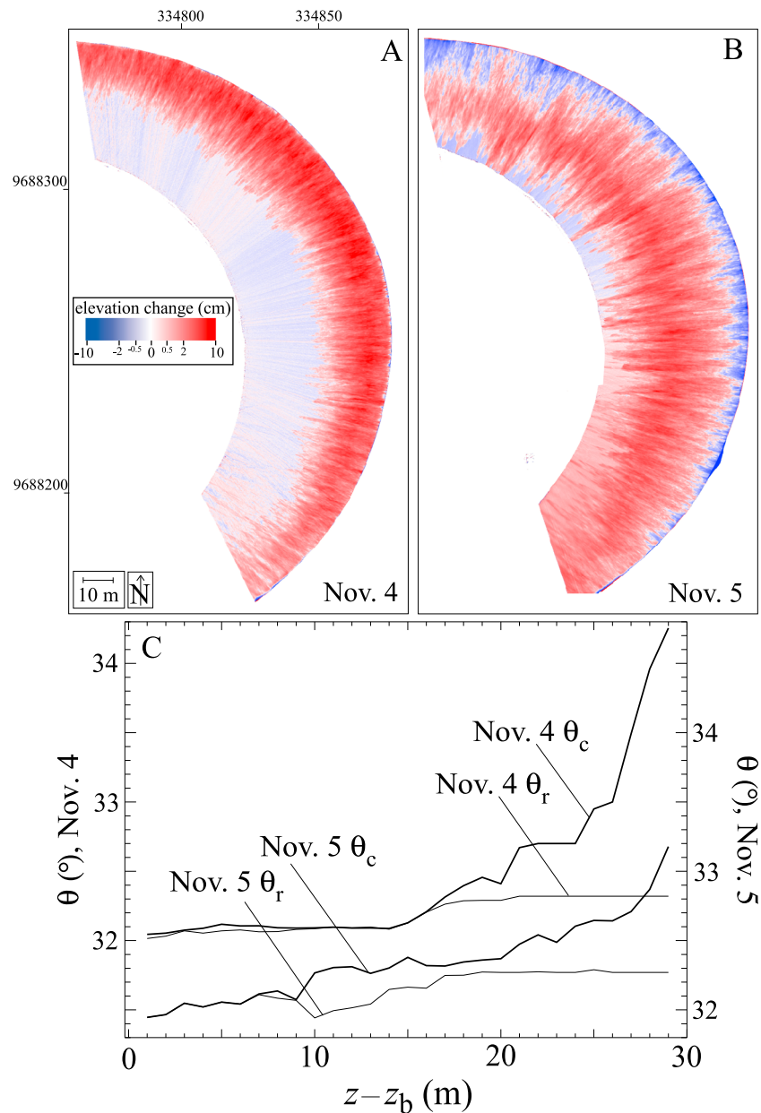
Figure 15. (a–c) Illustration of the effects of sand moisture on storage-and-release dynamics. A rainstorm on the morning of 4 November led to an approximately 1^\circ increase in \langle\theta_c\rangle (Figure 15c). The result of this increase is that no grain flows occurred on that day, only aggradation of the upper portion of the slope. After some drying of the sand occurred, the \langle\theta_c\rangle value decreased, which triggered sediment redistribution from the upper portion of the slope to the middle and bottom portions by grain flows.
