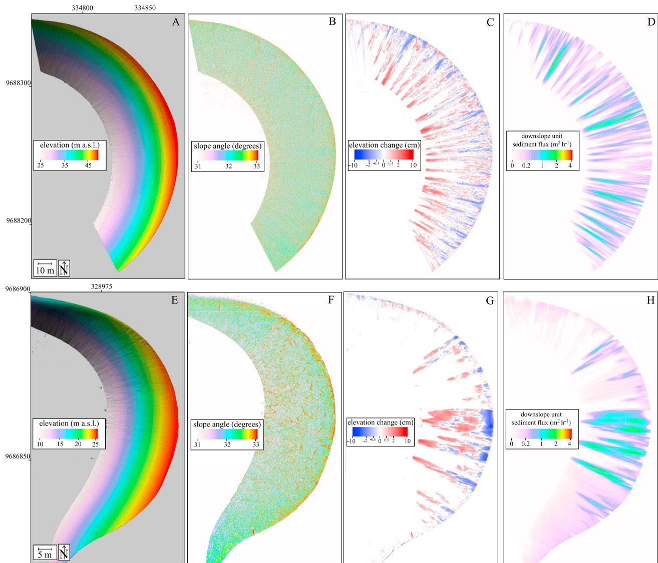
Figure 6. Color maps illustrating the types of data derived from terrestrial laser scanning (TLS). (a–d) Data for the large dune; (e–h) data for the small dune. Shaded-relief and color maps of slip-face elevations (Figures 6a and 6e), slope angles (Figures 6b and 6f), elevation changes over a 15 min interval (Figures 6c and 6g), and unit sediment fluxes (Figures 6d–6h) corresponding to the same intervals as Figures 6c and 6g.
