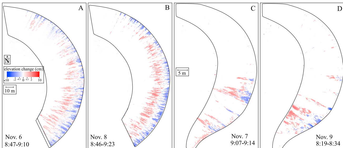
Figure 10. Color maps of topographic change for the first survey of the morning on each of the four dry days, illustrating the predominance of grain-flow activity on the southern portion of the dunes in the morning in the approximately 08:00–10:00 time interval. (a and b) large dune; (c and d) small dune. The approximate slip-face outline is shown in black.
