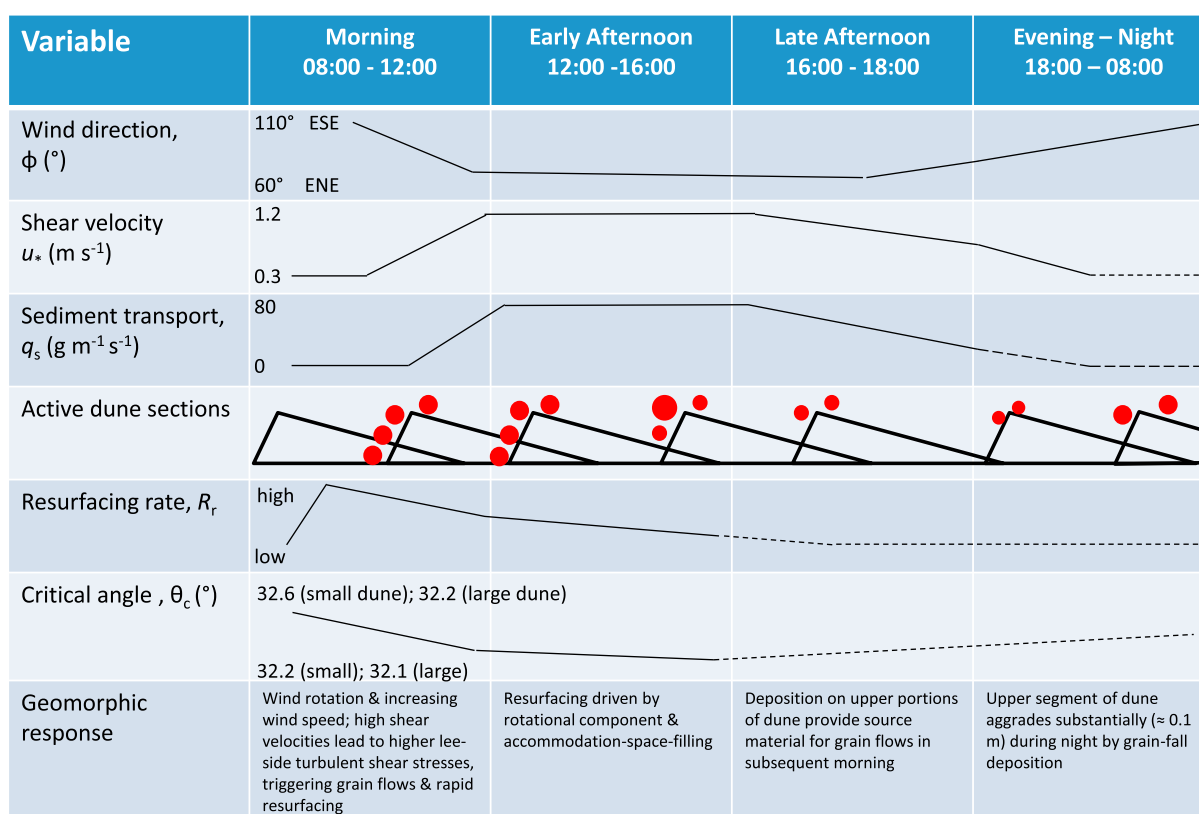
Figure 16. Summary of key variables of slip-face evolution and their diurnal variations at the study site under dry conditions.
