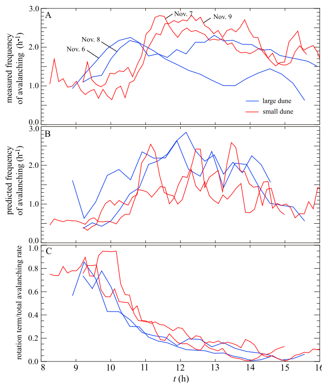
Figure 12. Plots of (a) measured frequency of avalanching, (b) predicted frequency of avalanching (from equation (8)), and (c) the ratio of the rotational component of the frequency of avalanching to the sum of the rotational and accommodation-space-filling components.
