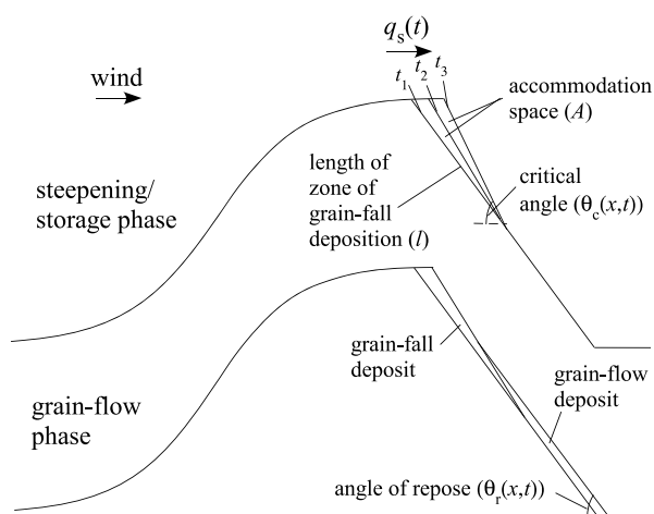
Figure 1. Schematic cross-sectional diagram of storage-and-release dynamics associated with dune slip-face evolution. In the steepening/storage phase, grainfall deposits accumulate on the upper portion of the slip face until a critical angle, \theta_c , is reached, at which point a grain flow is triggered. In the grain-flow phase, a portion of the grain-fall deposit is advected down the slope and deposited at the angle of repose, \theta_r , that is lower than \theta_c . The periodicity of cycles of storage and release is hypothesized to depend on the difference between the critical angle and the angle of repose (defined herein as the relaxation angle), as well as on the sediment flux over the brinkline, q_s . In addition, we hypothesize that a decrease in \theta_c with time can trigger grainflow activity independent of q_s .
