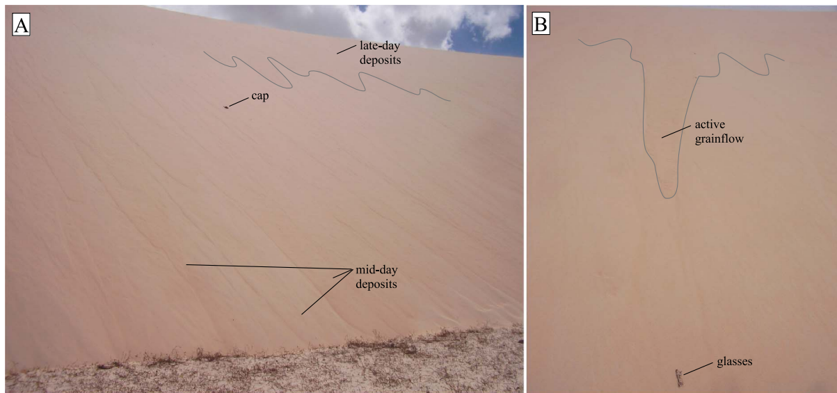
Figure 9. Field photographs illustrating (a) the multiple generations of deposits and (b) the morphology of an active grainflow.
