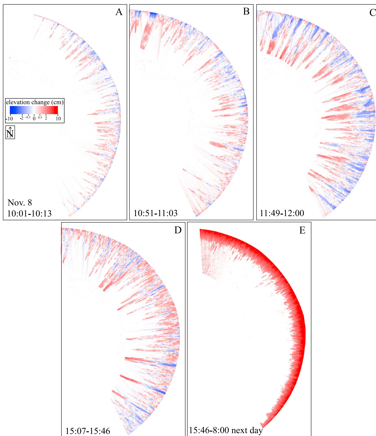
Figure 8. Color maps of elevation changes for select intervals of a dry day on the large dune (8 November).
