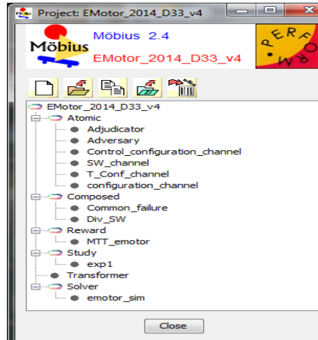
Fig. 2. The SAN project, E-Motor_2014_D33.
