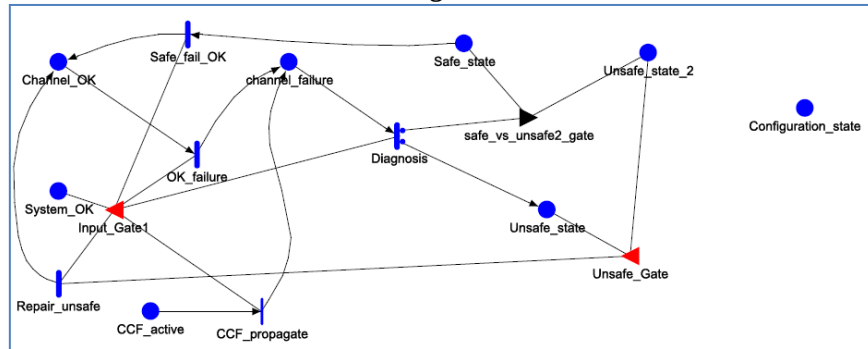
Fig. 4. Model of a SW channel
