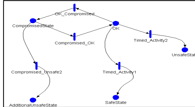
Fig. 1. A simplified SAN model of a channel of the E-motor
