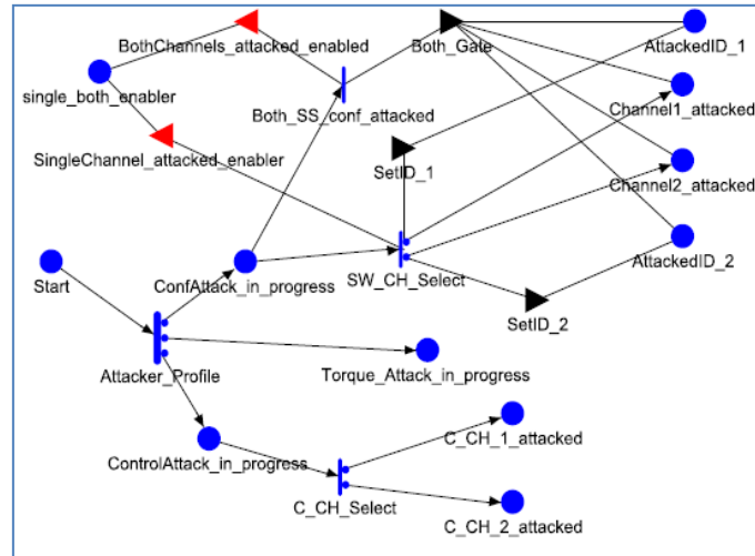
Fig. 5. A SAN model of the adversary
