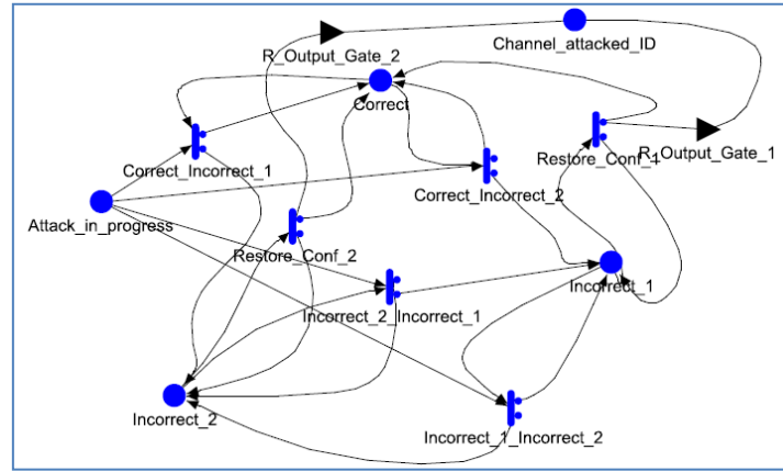
Fig. 6. A state model of a channel's safe state configuration file.
