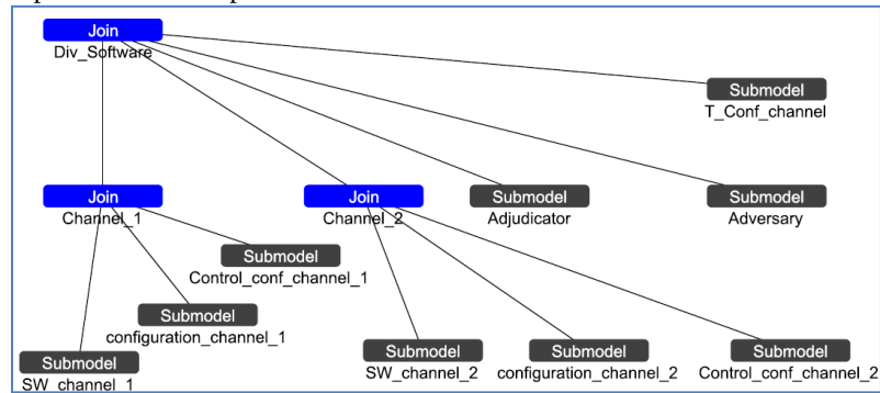
Fig. 3. The structure of the composed model, Div_SW
