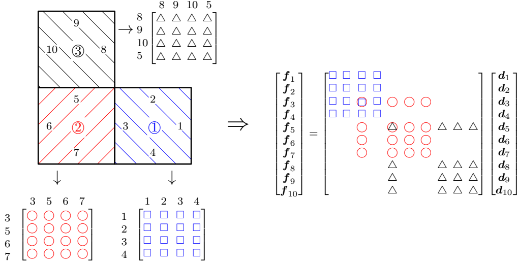
Figure 3: Illustration of the assembly procedure of a L-shaped plate assembly.
