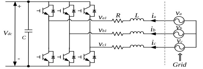
Fig. 2 Grid-connected converter schematic
