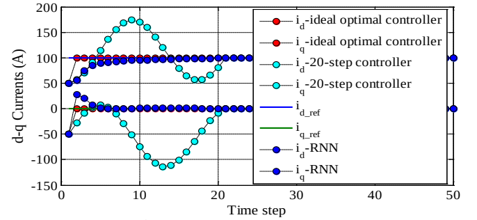
Fig. 12 Controller performance comparison between ideal optimal controller, 20-step controller and RNN controller.
