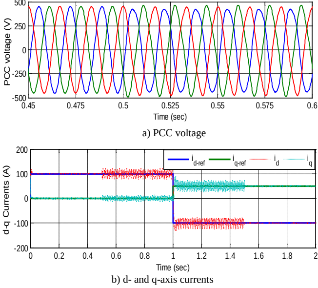
Fig. 16 d-q current under distorted grid voltage
