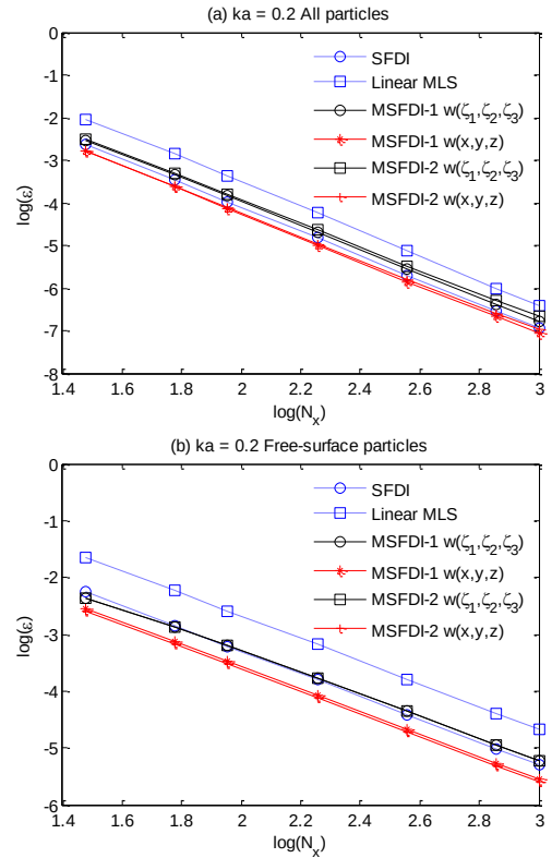
Figure 4: Convergent rate of gradient estimation for kh=2 and ka = 0.2 (quasi-uniform distribution, N_l=2 , \gamma=k )
