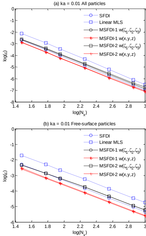
Figure 3: Convergent rate of gradient estimation for kh=2 and ka = 0.01 (quasi-uniform distribution, N_l=2 , \gamma=k )
