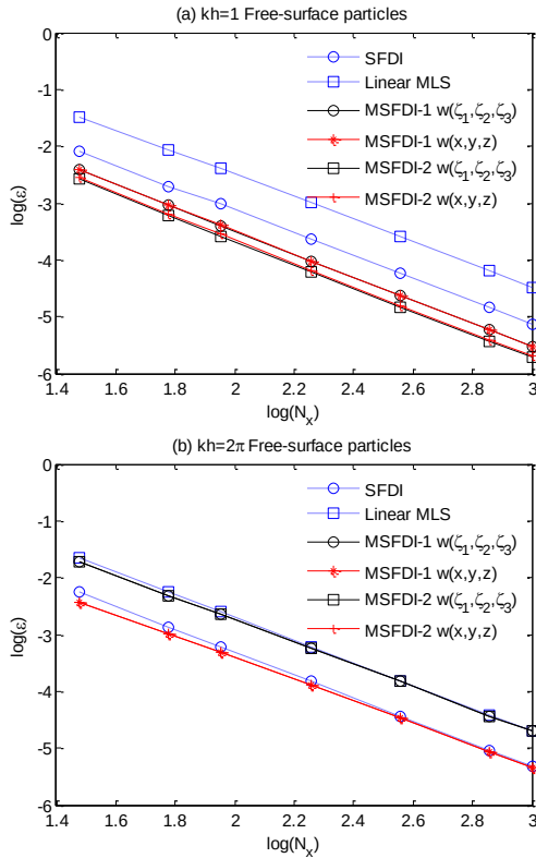
Figure 5: Convergent rate of gradient estimation for nonlinear regular waves ka = 0.2 (quasi-uniform distribution, N_l = 2 , \gamma = k )
