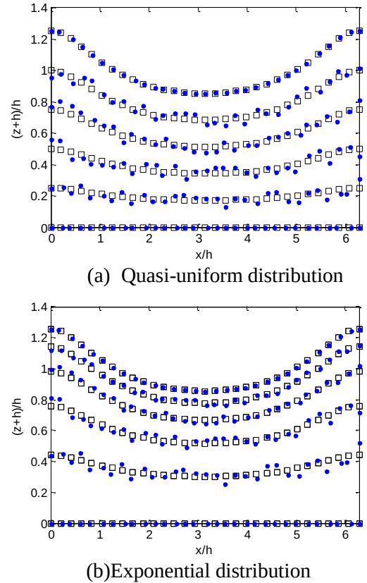
Figure 1: Example of distributions of particles (Hollow: initial distribution; Solid: with random shift)
