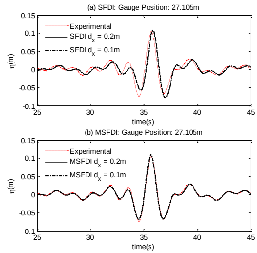
Figure 22: Comparison of the time histories of the wave elevations at x = 27.105\text{m} ( N_l = 1 , N_z = 20 )
