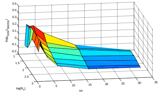
Figure 6: \log(\epsilon_{SFDI} / \epsilon_{MSFDI}) for free surface velocity estimations for nonlinear regular waves ka = 0.2 in the cases with different kh (quasi-uniform distribution, N_l = 2 , \gamma = k )
