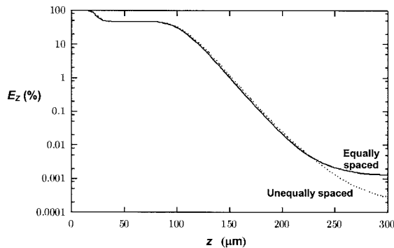
Fig. 6. Energy remaining in the real window, E_z (in %), as a function of propagation distance z . Results are shown for square profiles with unequally spaced and equally spaced distributions of sample points. The PML width is 6.7 \mu\text{m} (15% of the total window).
