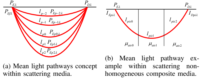
Fig. 2: “Banana” shaped light propagation envelope is split into smaller “canoe” shaped envelopes by the fraction of light going through them (Fig. 1a). Each smaller envelope can be approximated by the mean light pathway l_{pi} going through the smaller envelopes medians.
