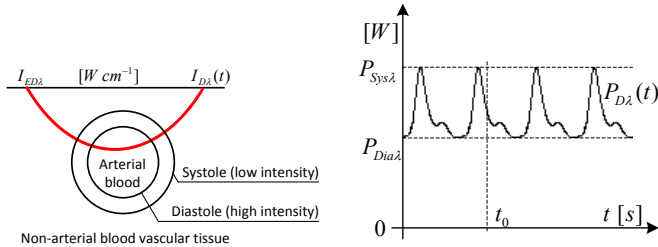
(a) Light-tissue interaction diagram during cardiac cycles—induced vascular tissue volume changes. (b) The PPG signal obtained from a tissue represented by the light-tissue interaction diagram on Fig. 3a.
