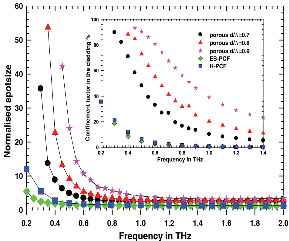
FIG. 6. Normalized spotsize variation with frequency for the porous fiber, the H-PCF and ES-PCF in Teflon.
