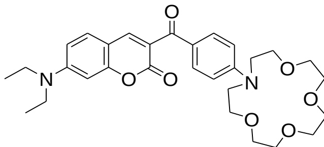
Fig. 4.5. Structural formula of the fluorescent molecule 1
