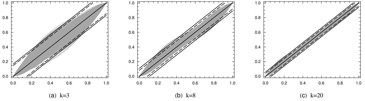
Figure 1: Graphs of 1000 simulations of \sum_{i=1}^p \xi_i N_{i,3}(t) , with \bar{\mathbf{t}}_{k,3} according to (20) and estimates of \hat{e}_{0.95} and \hat{\varepsilon}_{0.95} for: (a) p = 6 ( k = 3 ), \hat{e}_{0.95} = 0.17 , \hat{\varepsilon}_{0.95} = 0.18 ; (b) p = 11 ( k = 8 ), \hat{e}_{0.95} = 0.10 , \hat{\varepsilon}_{0.95} = 0.12 ; (c) p = 23 ( k = 20 ), \hat{e}_{0.95} = 0.05 , \hat{\varepsilon}_{0.95} = 0.07 .
