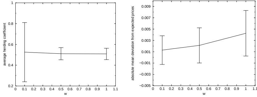
Figure 5: Average herding coefficient over time and the number of simulations as a function of w (left side). Deviation between realized prices and expected prices as a function of w (right side).
