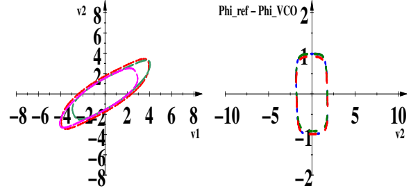
Figure 2: 3-Order \mathcal{AI} Projected onto (v_1, v_2) , and (v_2, (\phi_{ref} - \phi_{VCO}))
