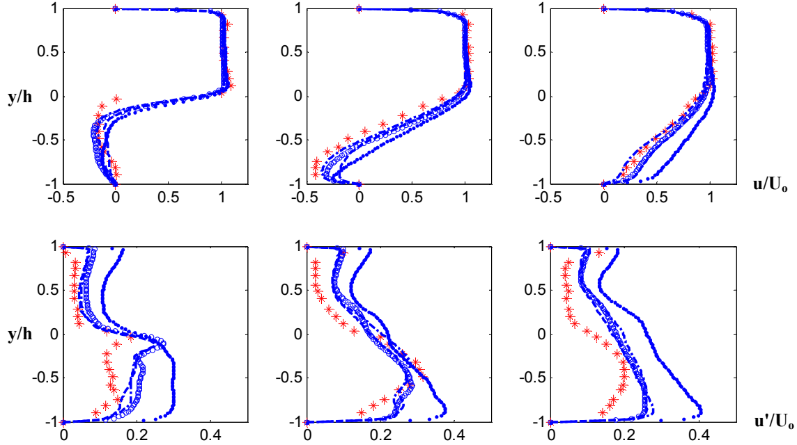
Figure 13: Normalized average/rms axial velocity profiles at x/H = 1, 3, 5 (reacting flow, coarse grid): *** Experiment, ••• LES (Colin-Algebraic, WD), ooo LES (Colin-Algebraic, JL), - - - LES (Charlette, JL), - · - · LES (Colin-Dynamic, JL)
