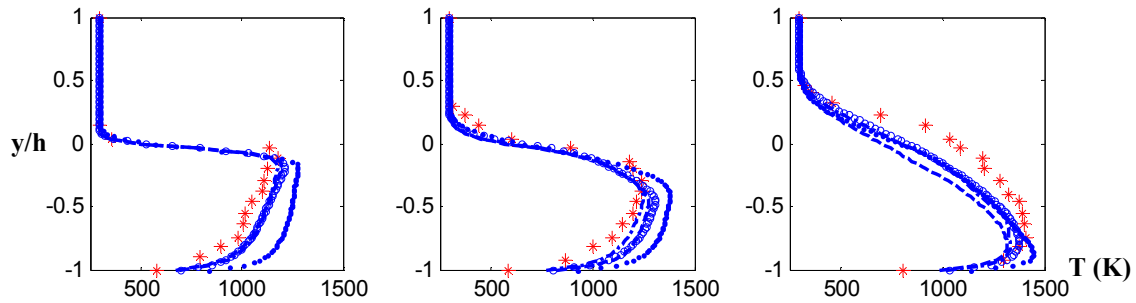
Figure 14: Average temperature profiles at x/H = 0.4, 1.2, 3.5 (reacting flow, coarse grid): *** Experiment, ••• LES (Colin-Algebraic, WD), ooo LES (Colin-Algebraic, JL), - - - LES (Charlette, JL), - · - · LES (Colin-Dynamic, JL)
