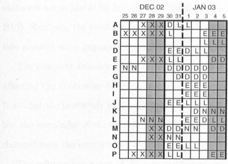
Figure 8.3: December-January continuity, “ORTEC01”
