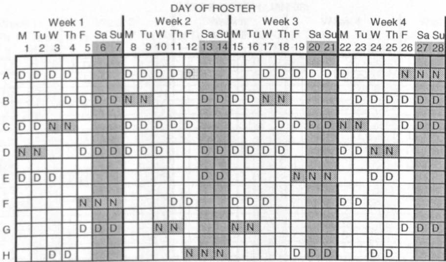
Figure 8.1: Optimal solution for problem “GPost”
