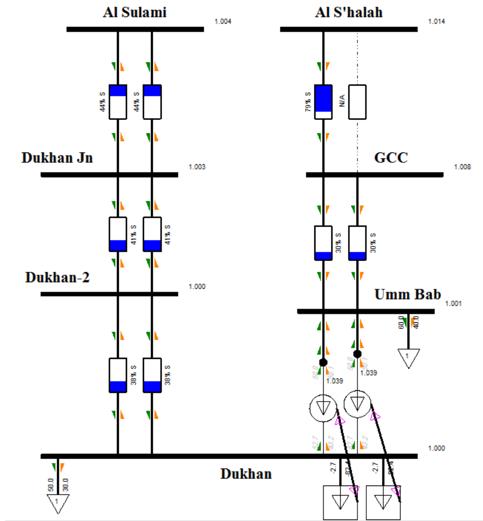
Figure 30: GUPFC (50 MW, 50 MVar)-Location-4, at Dukhan (towards Umm Bab)- N-1 at S'halah – GCC
