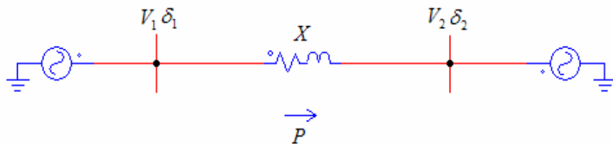
Figure 7: Typical power transmission line model
