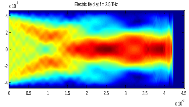
Figure 7. Electric field intensity distribution along the direction of propagation at 90% input pulse spot size.
