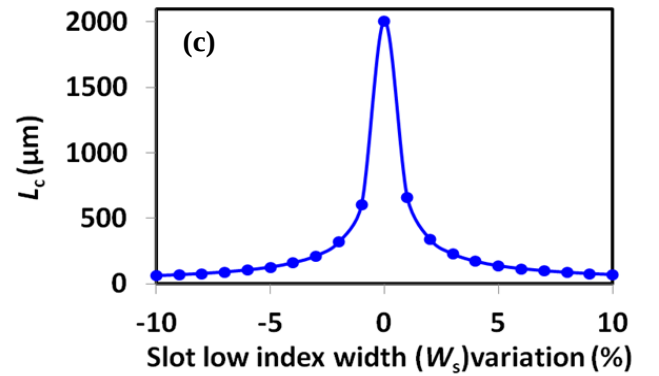
Figure 8. Tolerance study for L_c with the variation with slot parameter. (a) H variation; (b) W_2 variation; (c) W_s variation.
