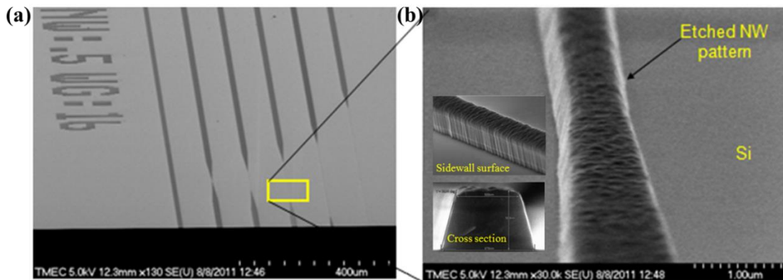
Figure 5: a) SEM image of nanowires in one set including two reference waveguides and four different lengths of nanowires. b) The magnification SEM image at the part of the nanowire involving the sidewall surface and cross section.
