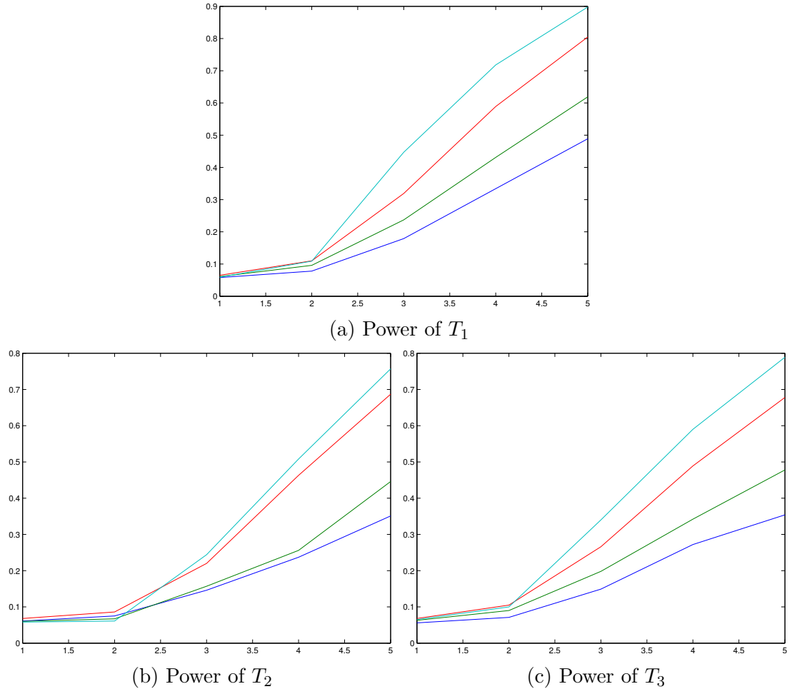
Figure 3: Power under different jump intensities. (a), (b), (c): n = 500 (blue), n = 1000 (green), n = 2000 (red), n = 3000 (cyan).
