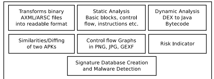
Fig. 8: Features of Androguard
