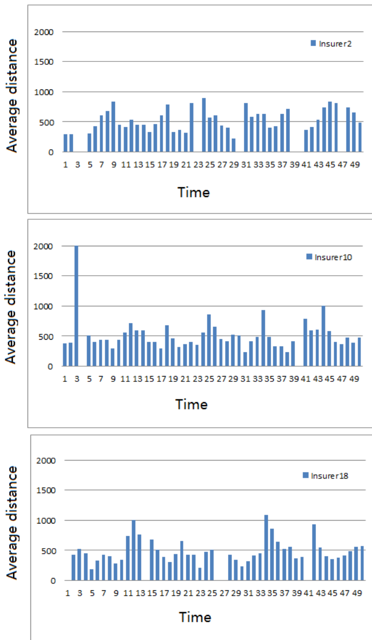
Figure 4.23: Average distance over 50 years
