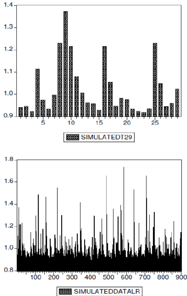
Figure 4.19: Model validation: simulated combined (or loss) ratios
