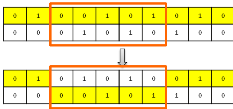
Figure 1-10: Crossover
