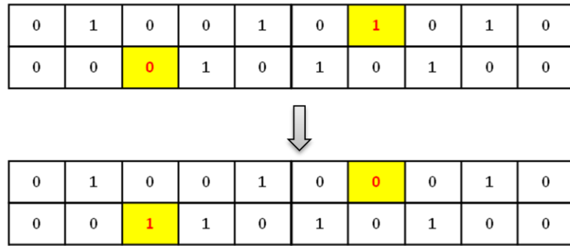
Figure 1-9: Mutation
