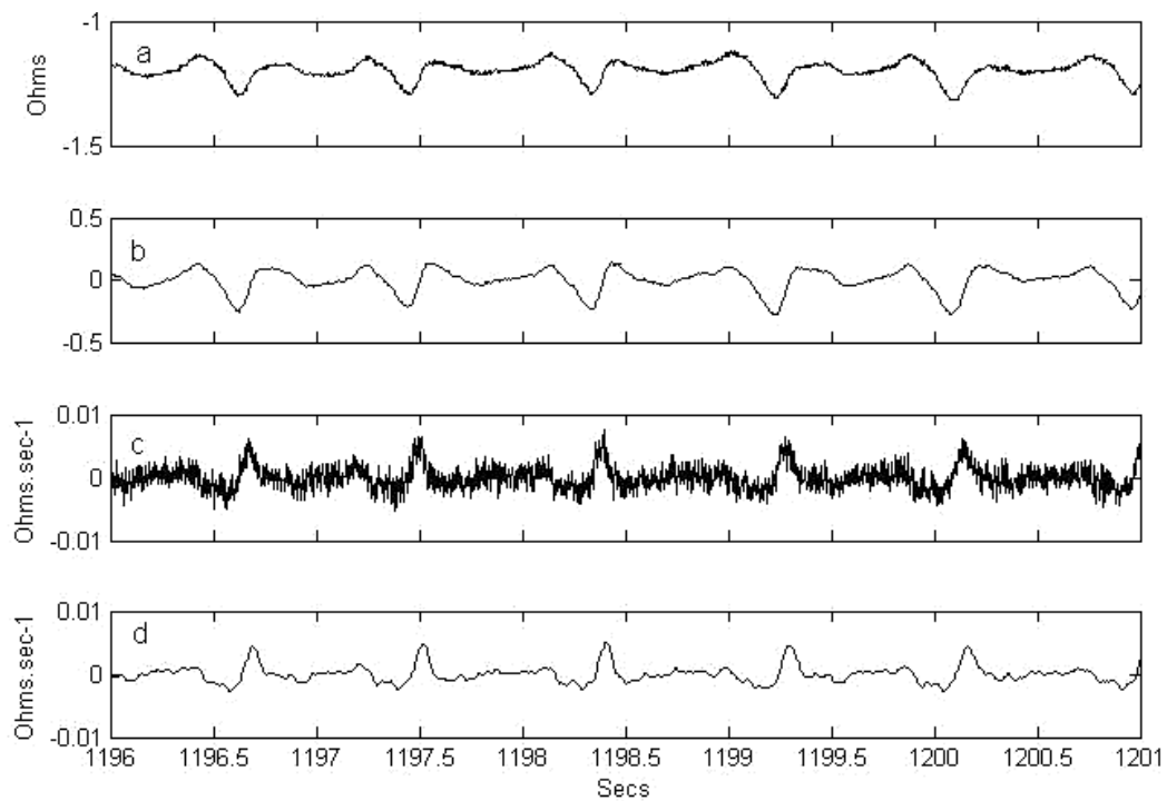
Figure 8.3 Stages in \Delta Z cardiac component signal processing. a) unfiltered \Delta Z ; b) \Delta Z with band-pass filtering; c) Differentiated \Delta Z ( dZ/dt ); d) dZ/dt with secondary low-pass filtering applied.
