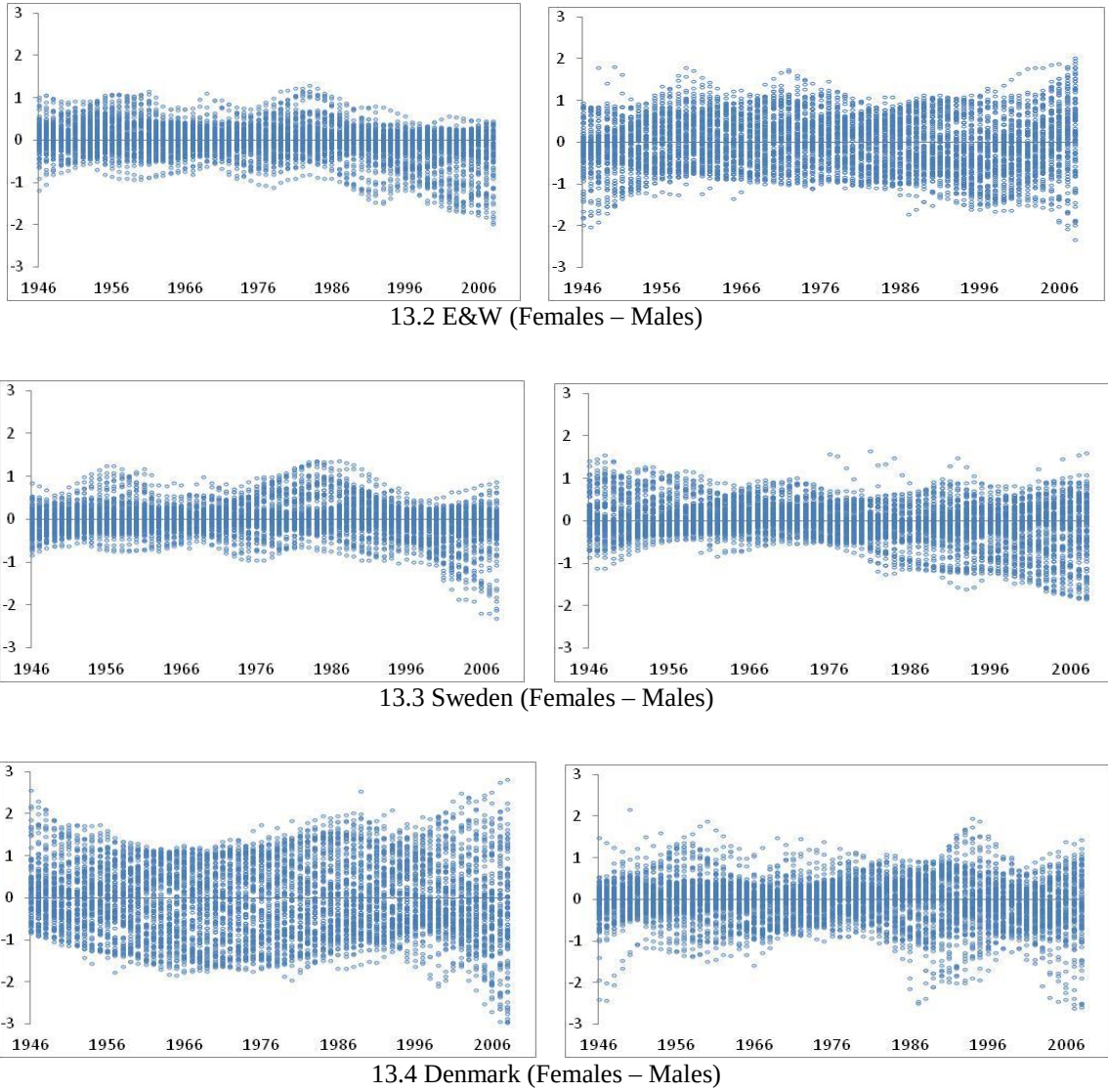
Figure 13: SDR vs. time effects for the age-cohort-period model (5), left graphs for females and right graphs for males.
