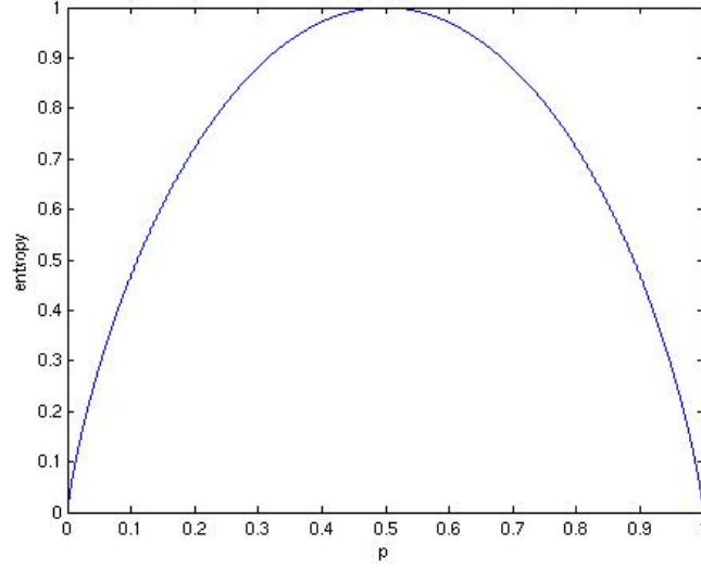
Figure 2.3: Concaveness of Entropy Function
