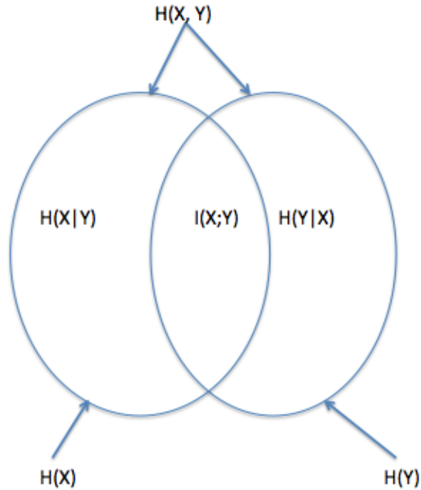
Figure 5.1: Relationship between entropy and mutual information
