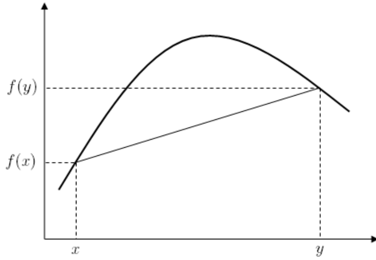
Figure 2.2: Example of Concave Function
