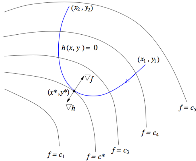
Figure 4.1: Lagrange multiplier Method
