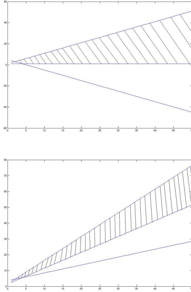
Figure 5.5: Polyhedron for Example 5.7.2 with horizontal axis being X and vertical axis being Y
