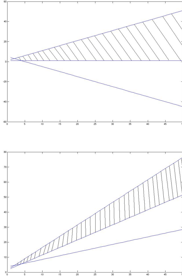
Figure 3.1: Polyhedron for Example 3.3.2 with horizontal axis being X and vertical axis being Y
