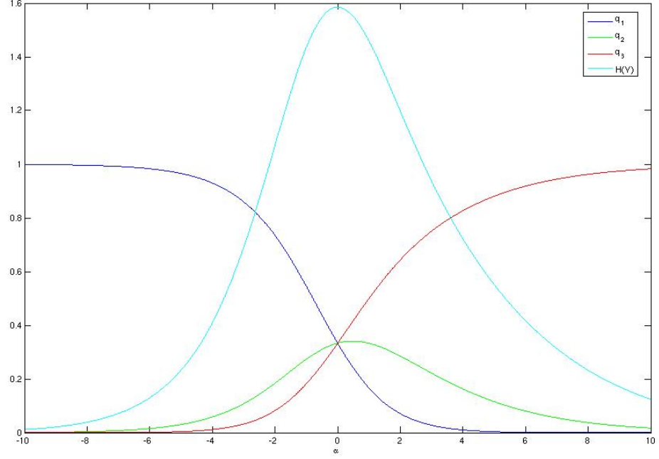
Figure 5.2: Marginal Probability Distribution and Marginal Entropy in terms of \alpha
