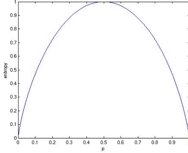
Figure 6.1: Concaveness of Entropy Function
