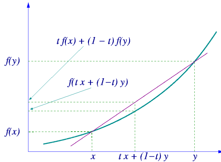
Figure 2.1: Example of Convex Function
