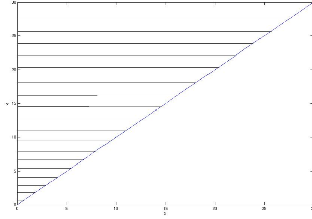
Figure 3.2: Polyhedron for Example 3.3.3 with horizontal axis being X and vertical axis being Y
