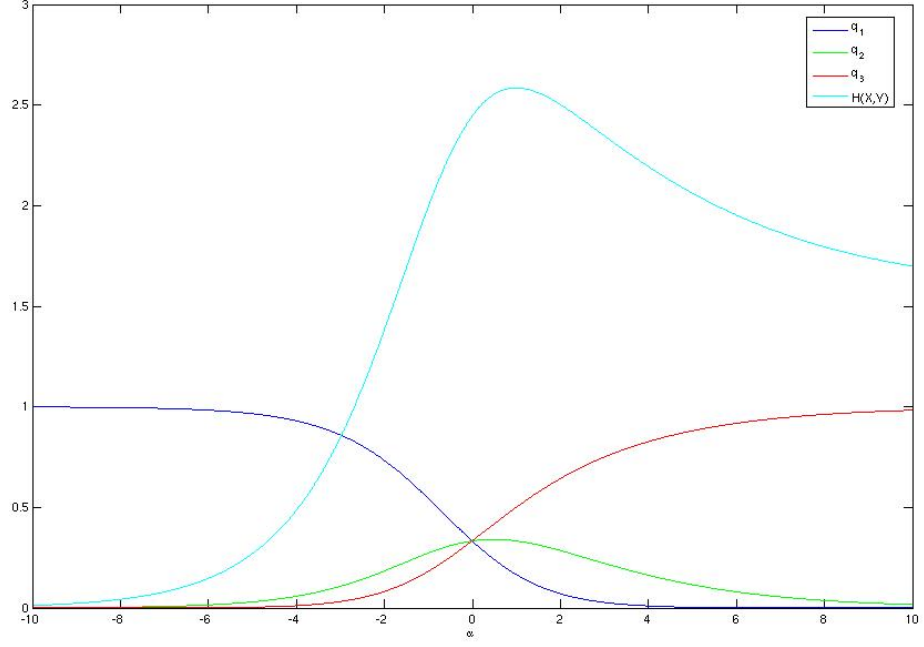
Figure 5.3: Marginal Probability Distribution and Maximal Joint Entropy in terms of \alpha
