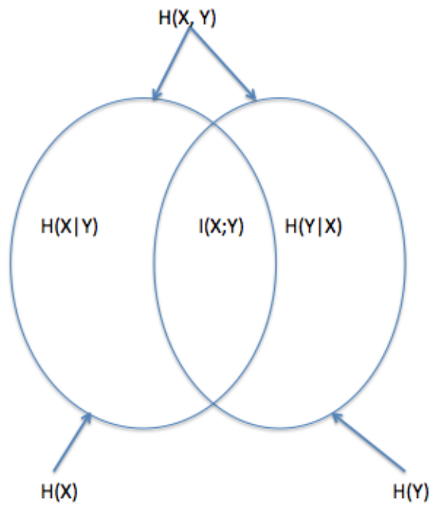
Figure 2.4: Relationship between entropy and mutual information
