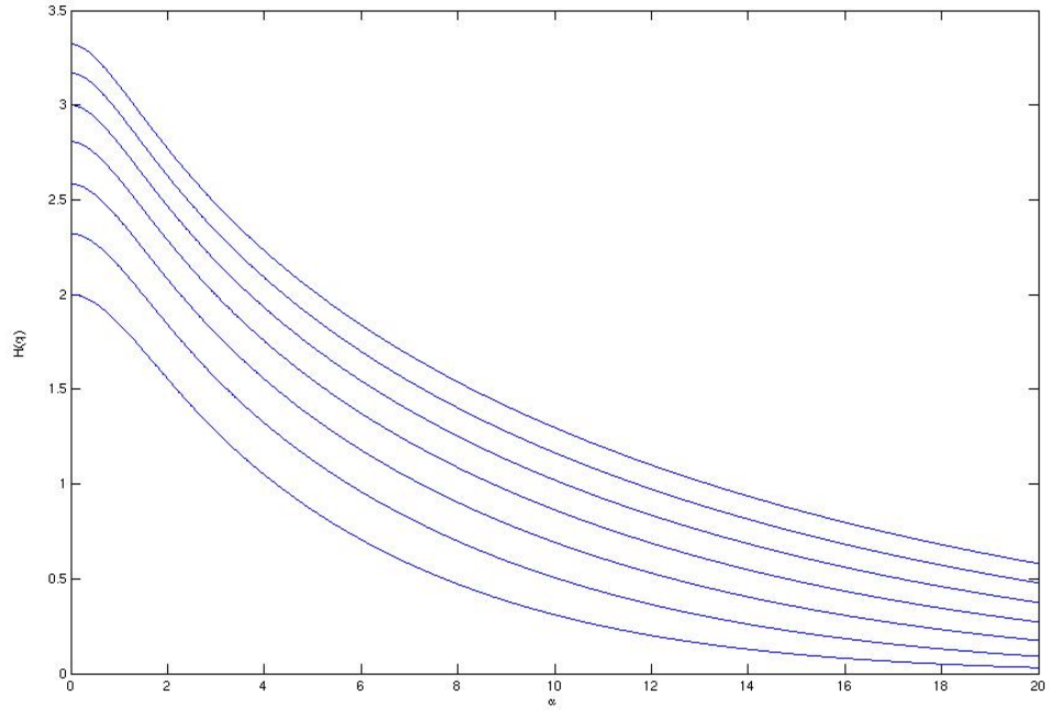
Figure 5.4: Marginal Probability Distributions of Different n : the bottom one is n = 4 , the top one is n = 10
